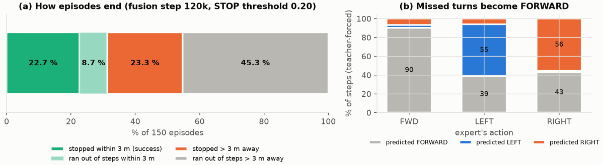
Figure 9: Pointing with layer fusion. (a) How the 150 episodes end. (b) Teacher-forced predictions by expert action: missed turns become FORWARD.
