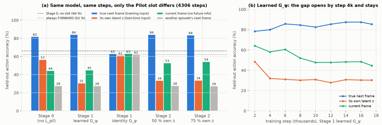
Figure 5: The Pilot-slot shortcut, measured. (a) Held-out action accuracy of each checkpoint with only the slot content changed. (b) The learned Stage 1 model over training: own-latent accuracy collapses by step 4k and stays low while next-frame accuracy stays high.
