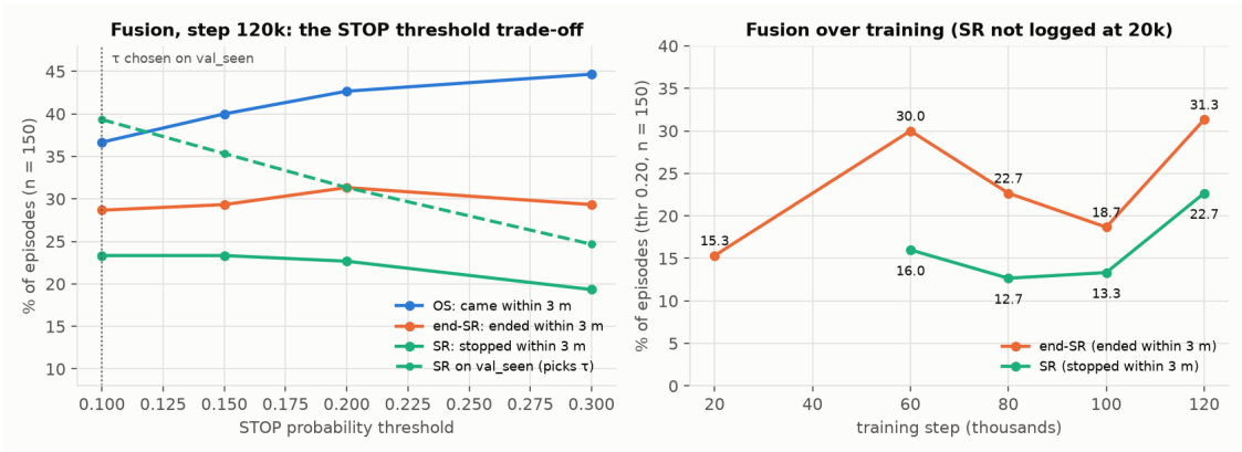
Figure 8: Pointing with layer fusion. Left: raising the STOP threshold \tau trades premature stops for overshoots. OS keeps rising, end-SR peaks at 0.20, and SR is flat up to 0.20 and then falls. Right: end-SR and SR over training at \tau=0.20 (stopping positions were not logged at 20k).
