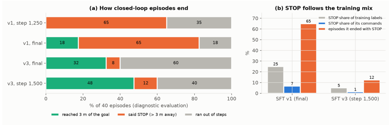
Figure 12: Reasoner. (a) How the 40 closed-loop episodes end (diagnostic evaluation). (b) STOP behaviour follows the STOP share of the training labels.
