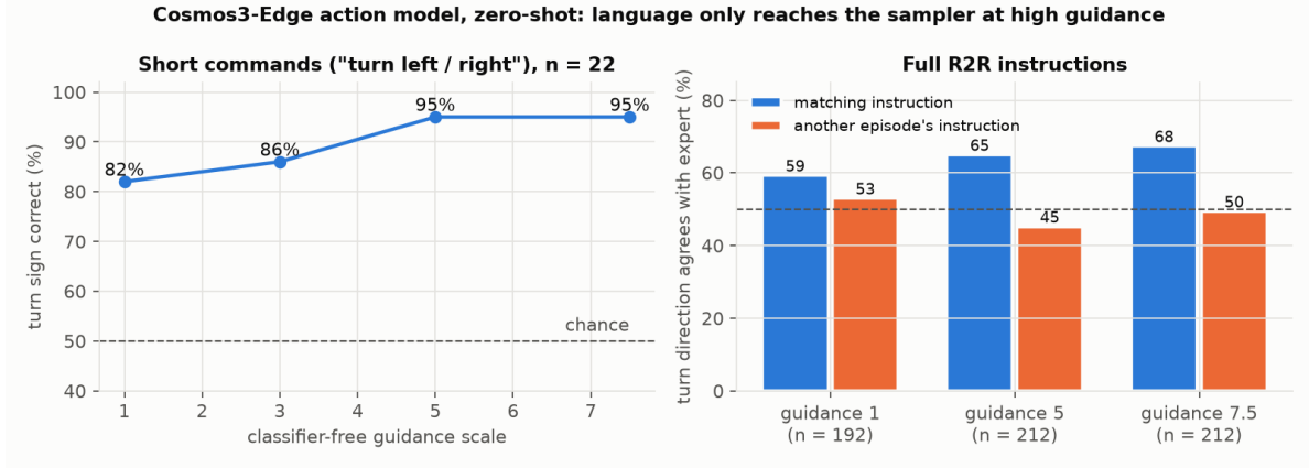
Figure 10: Cosmos3-Edge action model, zero-shot. Language influences the sampled motion only at high classifier-free guidance, and full instructions steer it weakly.
