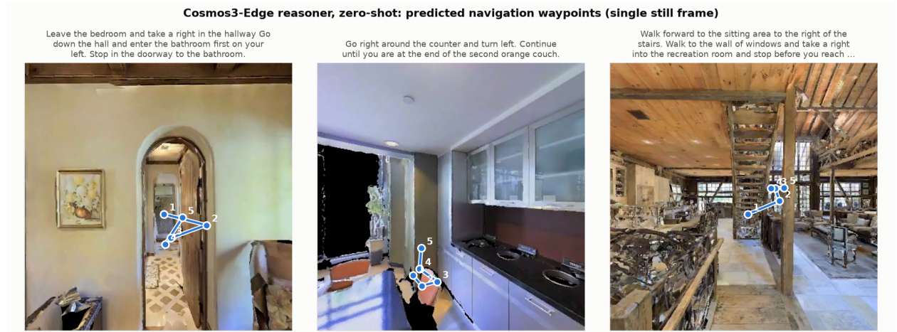
Figure 11: Zero-shot reasoner: predicted navigation waypoints on single frames (coordinates normalised to 0-1000).
