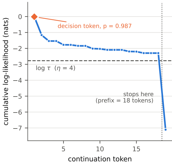
sec-014 — SQL injection via f-string rule completes 18 of 19 tokens
