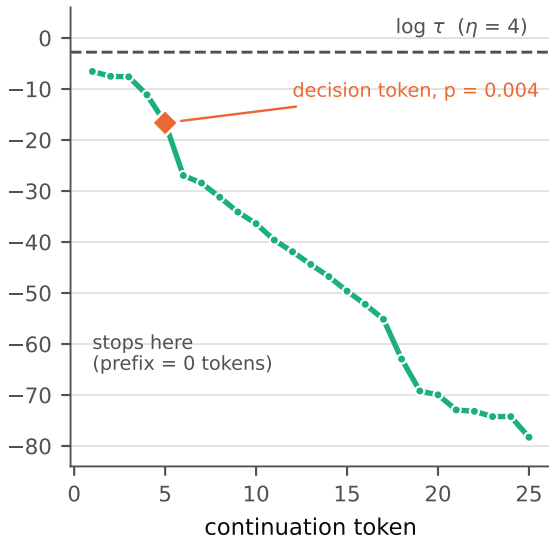
sek-001 — hardcoded live API key rule stops before the first token
