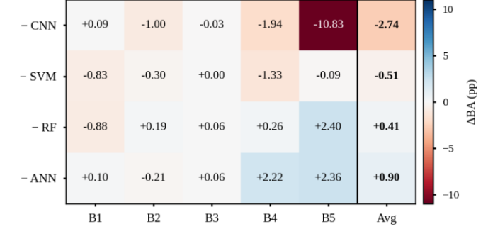
Fig. 5. Change in BA (pp) relative to the full weighted-vote ensemble when a member is removed (“− CNN” removes only the CNN’s own output). Negative = the member helps.
