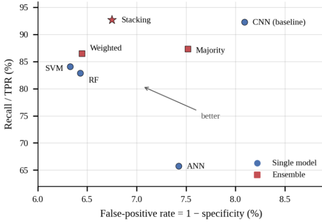
Fig. 4. Average operating points (mean over five benchmarks). Stacking is the only ensemble that improves on the CNN in both recall and false-positive rate.
