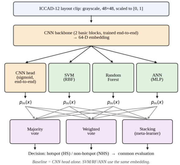
Fig. 1. Proposed ensemble. All four heads use the same 64-D CNN embedding; three combiners are compared with the CNN head alone.
