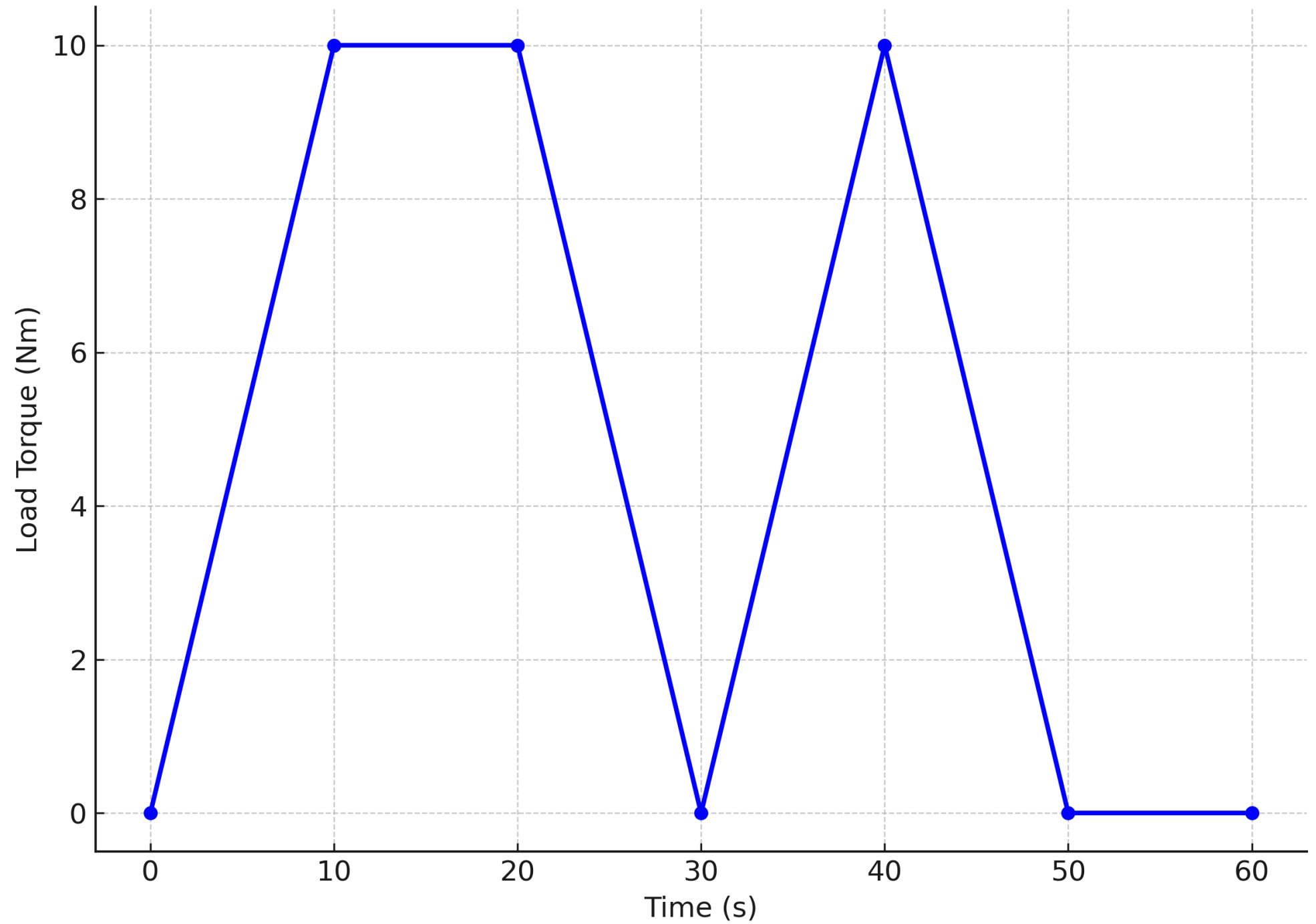
Load Torque vs Time
