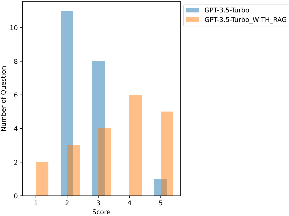
Question Wise Score Comparison For GPT-3.5-Turbo Model
