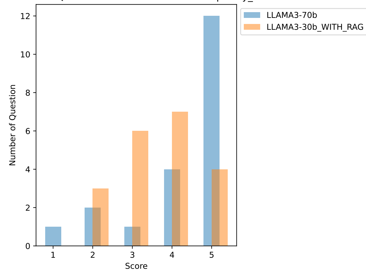
Number of Question VS Score Plot For Cyber_crime
