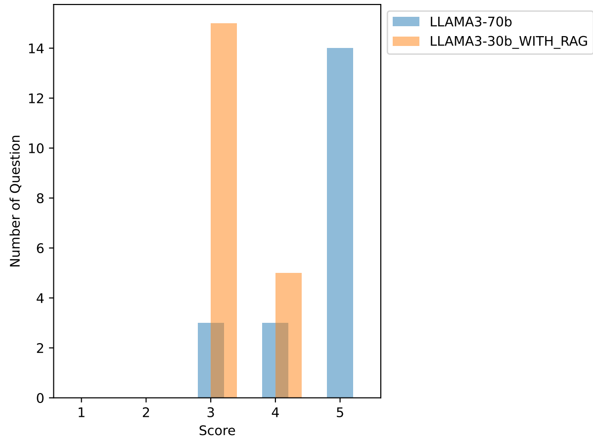
Number of Question VS Score Plot For Juvenile
