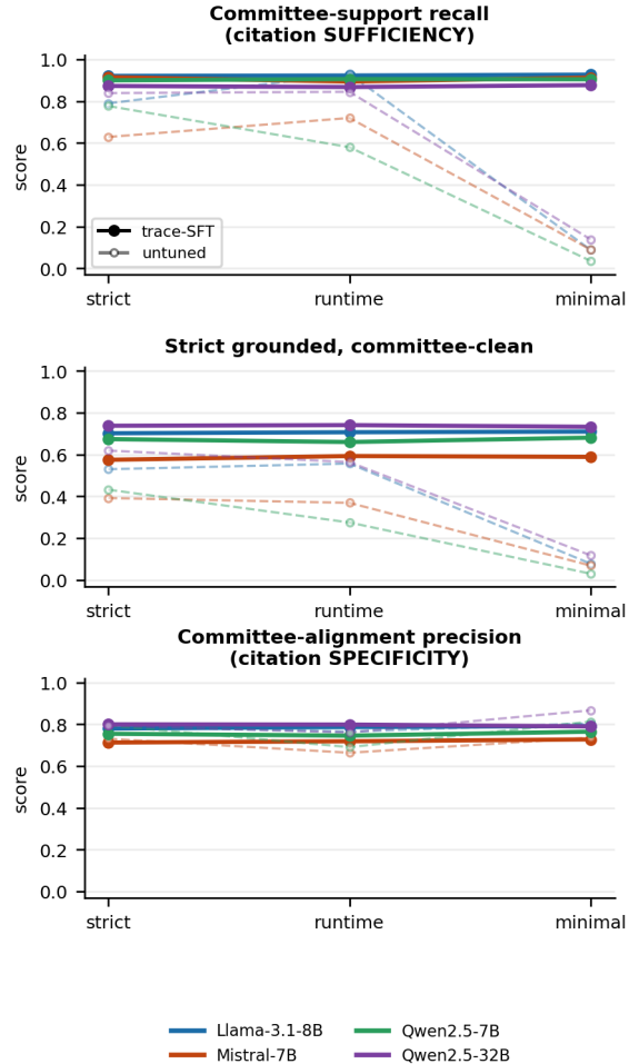
Figure 9: Trace supervision fixes citation sufficiency, not citation precision.
