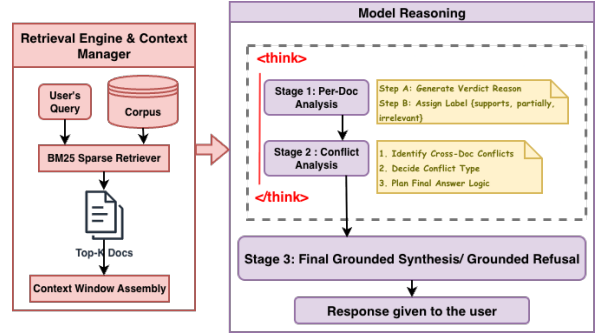
Figure 1: The evidence trace. The model adjudicates each retrieved document, infers the cross-document conflict pattern and produces a conflict-conditioned grounded answer or a justified refusal. Every stage is emitted in a machine-checkable form, so a downstream failure can be attributed to a stage rather than to the system as a whole.
