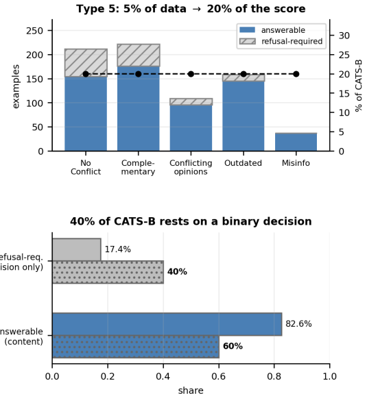
Figure 7: Structural properties of the aggregate.
