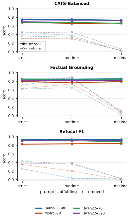
Figure 13: Behaviour across the prompt ladder. Solid lines are trace-tuned models, dashed lines untuned. Fine-tuned behaviour is essentially flat as the instruction is stripped away; untuned grounding and refusal collapse.
