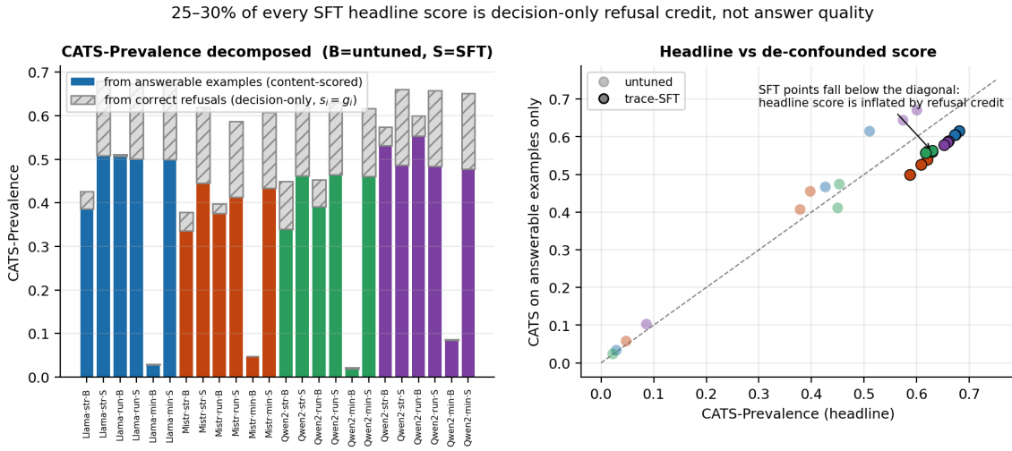
Figure 6: Refusal credit inside the aggregate. Left: CATS-Prevalence split into the part earned on answerable examples and the part earned on correct refusals, which are scored on their decision alone. Right: plotting the answerable-only score against the headline places every trace-tuned point below the diagonal, showing the headline is inflated by decision credit.
