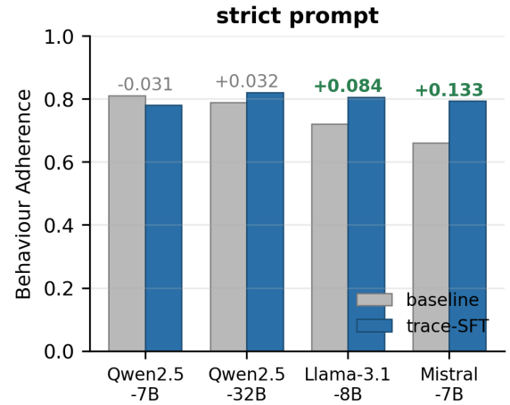
Figure 14: Behaviour Adherence under the strict prompt, baseline against trace-tuned. Deltas are annotated; bold green marks a gain exceeding the \pm 0.034 noise floor.
