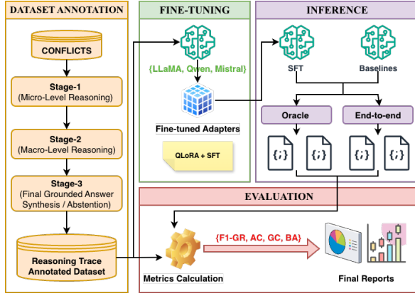
Figure 2: System overview. A weighted multi-annotator committee produces the supervision corpus; models are fine-tuned to emit the three-stage trace; CATS evaluates refusal calibration, conflict behaviour, factual grounding and answer recall, with an independent human study validating the automated judgements.
