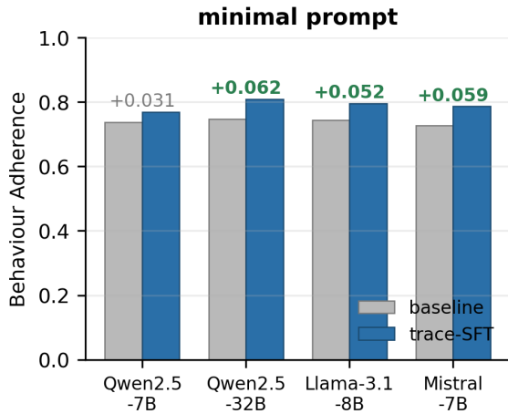
Figure 15: Behaviour Adherence under the minimal prompt. Baselines compress into a narrow band once the instruction no longer names the taxonomy, and every model gains.
