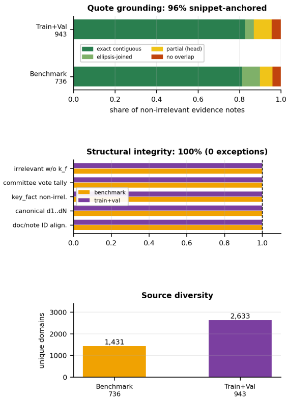
Figure 4: Quality audit computed directly from the released files.
