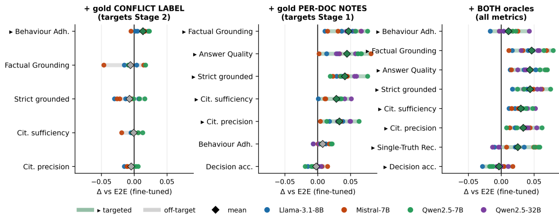
Figure 17: Each oracle moves the metric it targets and essentially nothing else. Green bars are targeted metrics, grey bars are specificity controls; diamonds mark means, points individual model × prompt cells.
