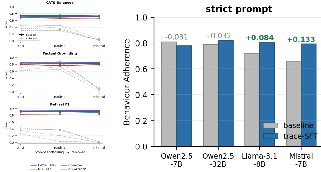
Figure 13: Behaviour across the prompt ladder. Solid lines are trace-tuned models, dashed lines untuned. Fine-tuned behaviour is essentially flat as the instruction is stripped away; untuned grounding and refusal collapse; Figure 14 : Behaviour Adherence under the strict prompt, baseline against trace-tuned. Deltas are annotated; bold green marks a gain exceeding the \pm 0.034 noise floor.
