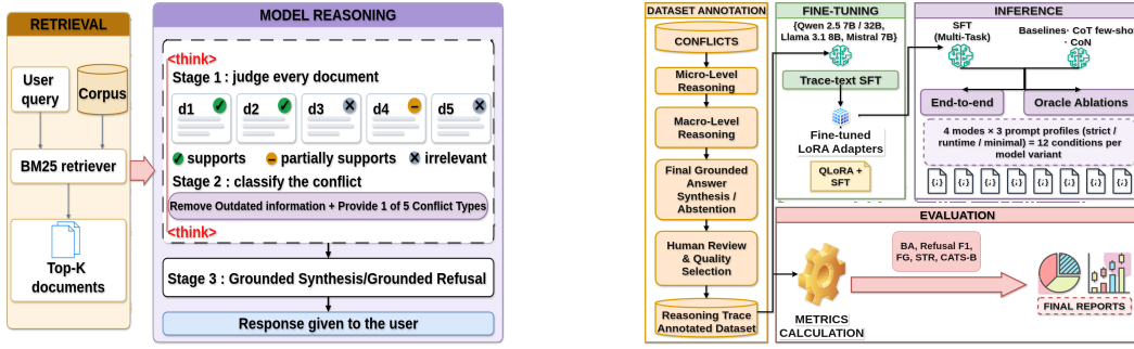
Figure 1: The evidence trace. The model adjudicates each retrieved document, infers the cross-document conflict pattern, and produces a conflict-conditioned grounded answer or a justified refusal; Figure 2: System overview. A weighted multi-annotator committee produces the supervision corpus. Models are fine-tuned to emit the three-stage trace. CATS evaluates grounded refusal, behavioural adherence, factual grounding, and single-truth recall, with an independent human study validating the latter three. We compute grounded refusal deterministically.
