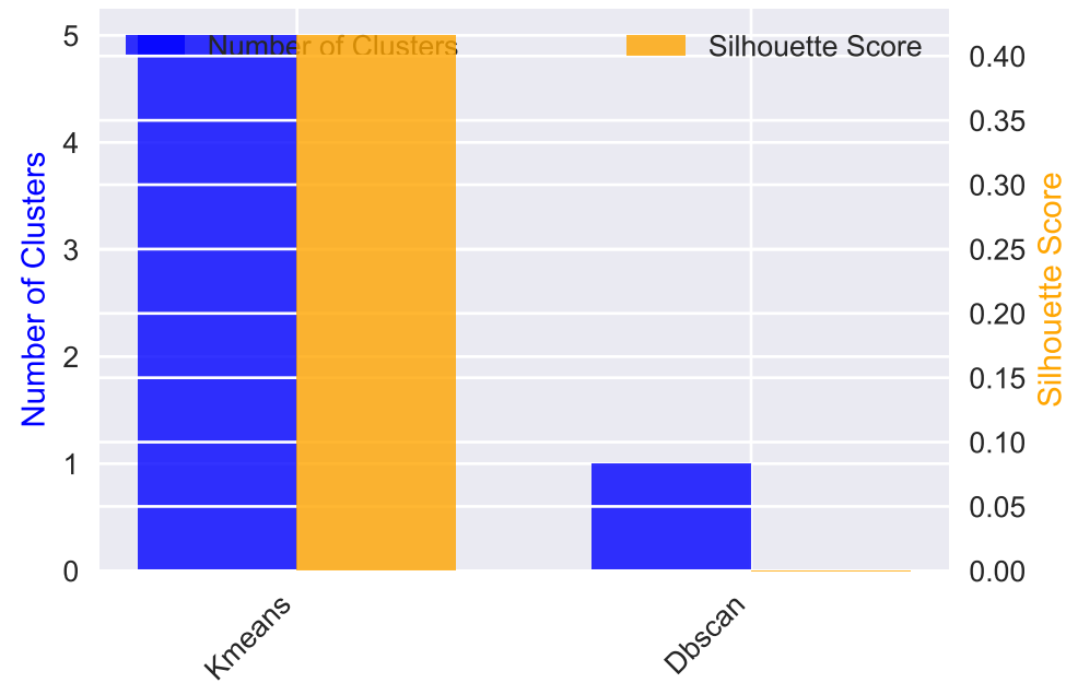
Cluster Visualization
