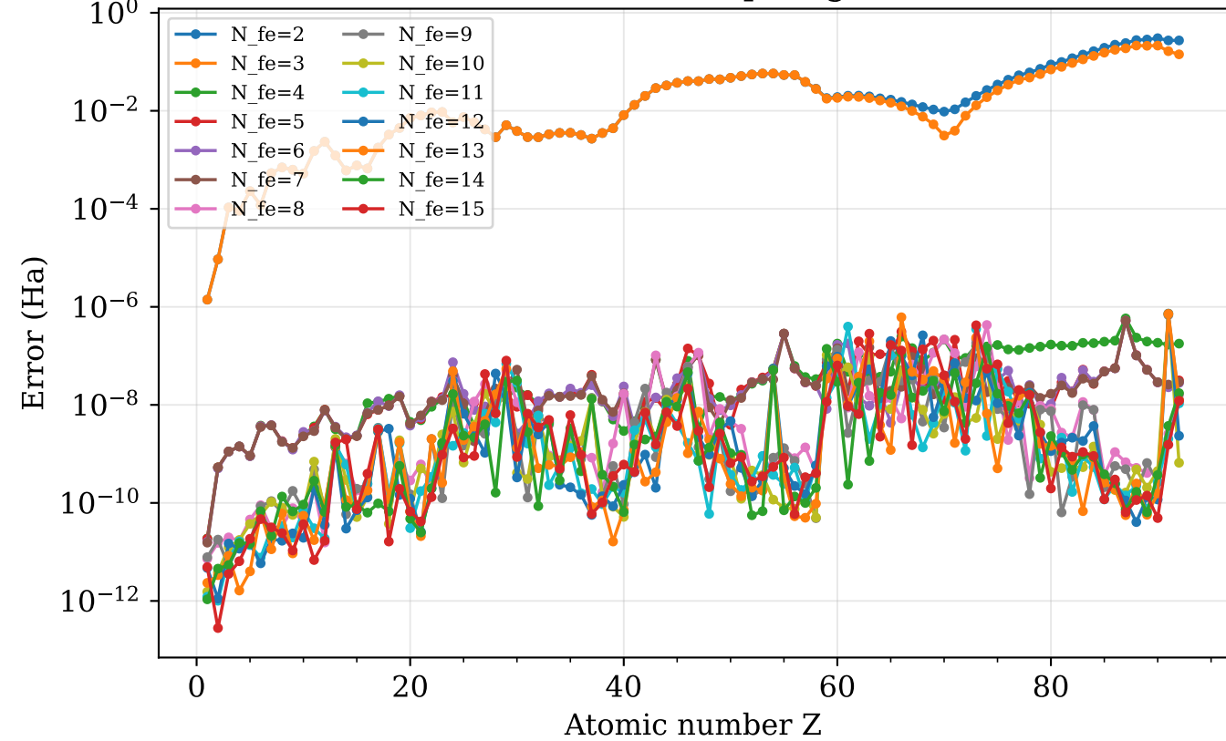
Finite-element sweep: Eigenvalues
