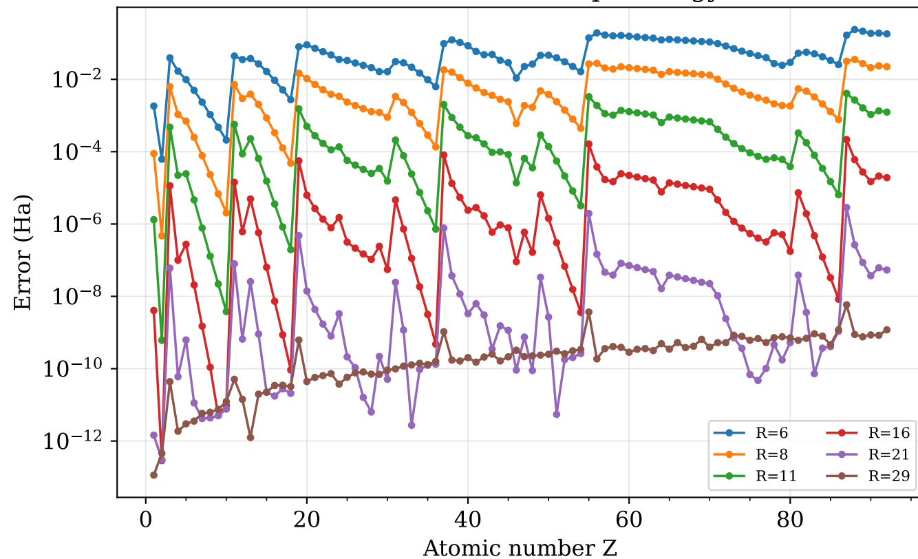
Finite-element sweep: Energy
