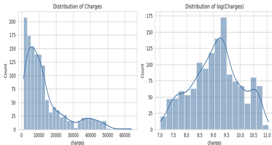
Figure 1: Distribution of raw charges (left, right-skewed) vs. log-transformed charges (right, closer to normal).
