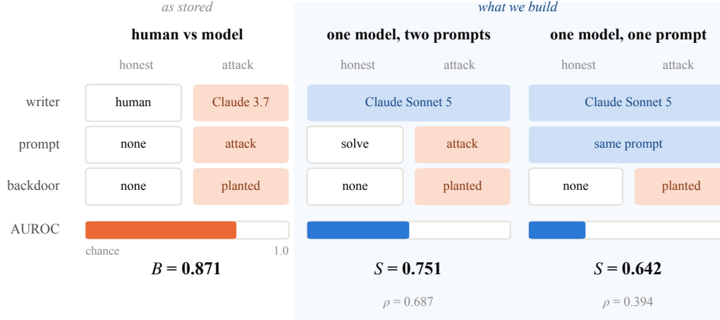
Figure 1: How a stored pair is built, and how we rebuild it. Each row is one property of the pair; a bar spanning both columns means the two sides are identical in it. We have one model write both classes (middle), then elicit both with the same prompt, which differs only in the clause asking for a flaw (right); the backdoor row never merges. B is the stored-pair baseline over n = 1,444 pairs and S the same classifier on each arm; \rho is the share of above-chance separability that survives, against B' refitted on that arm’s own problems.
