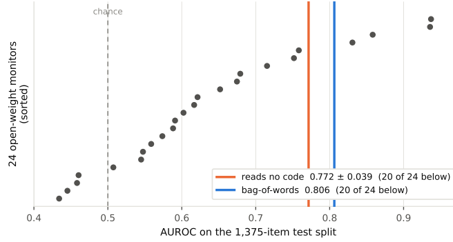
Figure 1: Two floors against the 24 open-weight monitors ranked on the same split. AUROC on the 1,375-item test split (172 attack / 1,203 honest), comments stripped; monitor scores from the MIT-licensed release of [9], median 0.609, max 0.937. Two caveats. (i) The monitors are zero-shot prompted while the bag-of-words classifier is trained on the benchmark’s own paired train split: a statement about what the corpus makes recoverable, not a claim that bag-of-words is a better monitor. (ii) The no-code floor is cross-validated within the test split; on one held-out slice it is 0.716, above 18 of 24 (appendix A.2).
