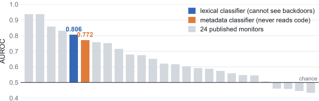
AUROC on the filtered test split
