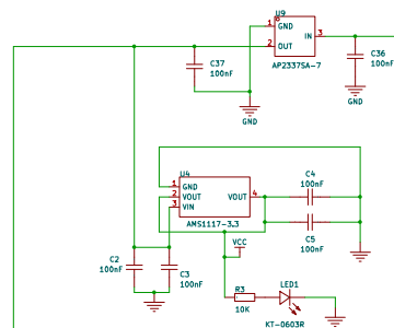
Voltage Regulator
