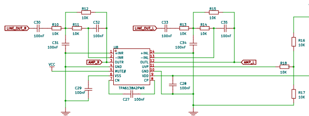
Headphone Amp
