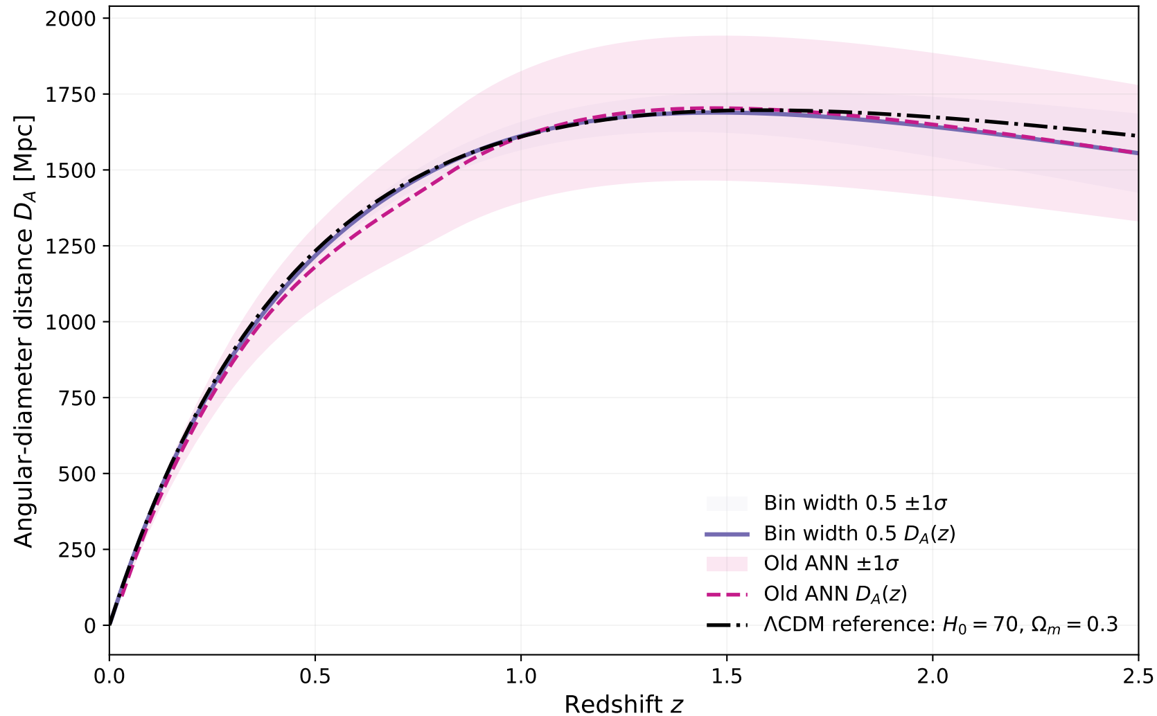
D_A(z) from binned-CV width 0.5, old ANN, and \Lambda CDM
