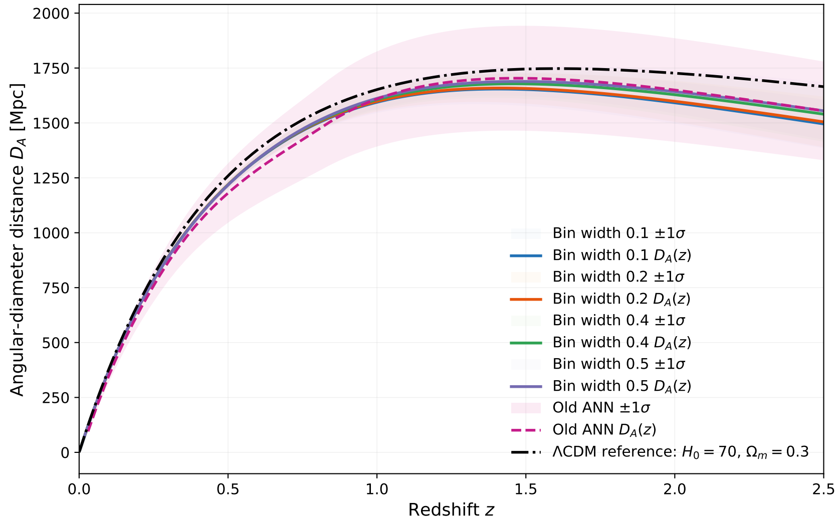
D_A(z) from four binned-CV widths, old ANN, and \Lambda CDM
