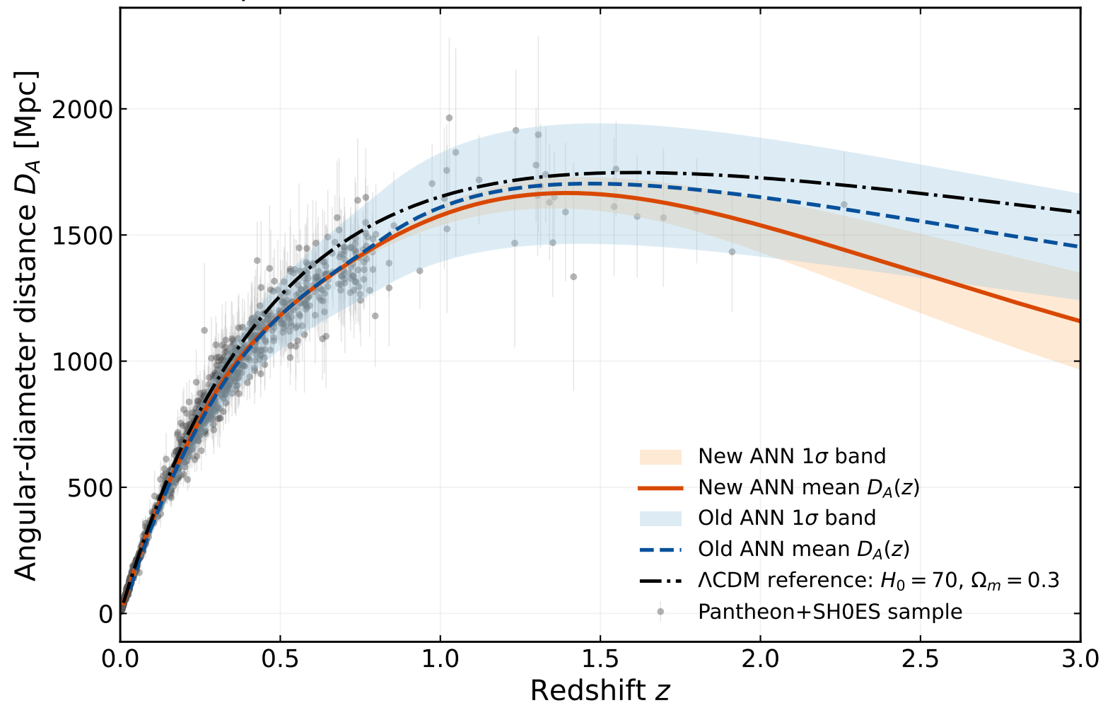
Comparison of old and new ANN reconstructions of D_A(z)
