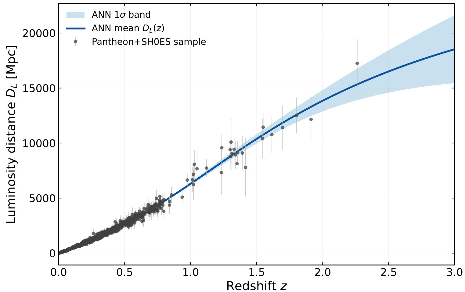
Pantheon+SH0ES ANN reconstruction of D_L(z)
