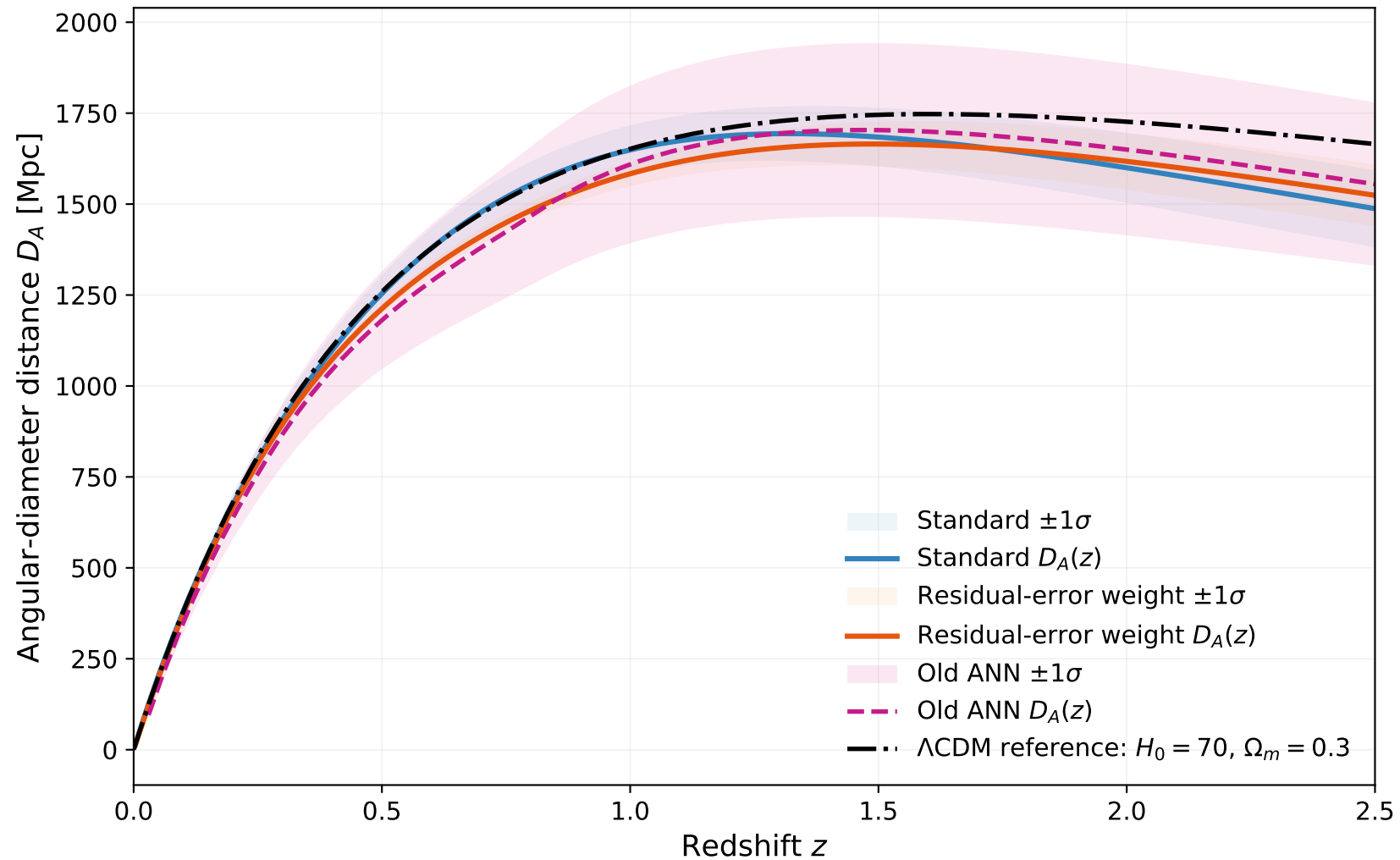
D_A(z) from two residual-space modes, old ANN, and \Lambda CDM
