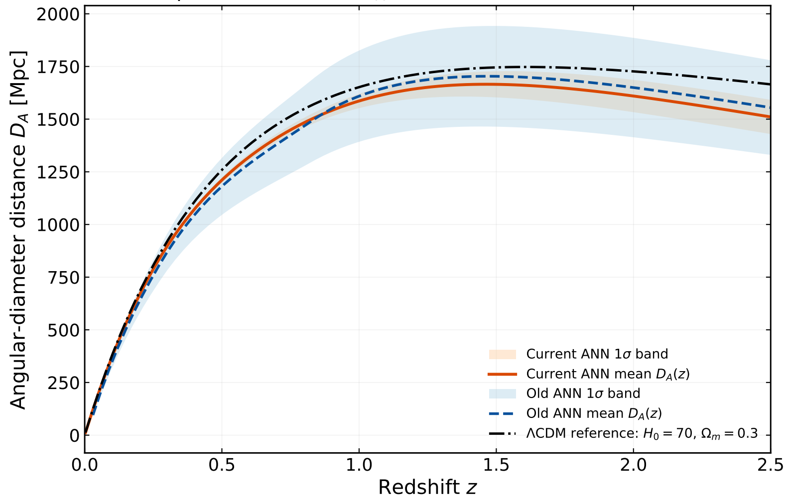
Comparison of current D_A(z) , old ANN, and \Lambda CDM reference
