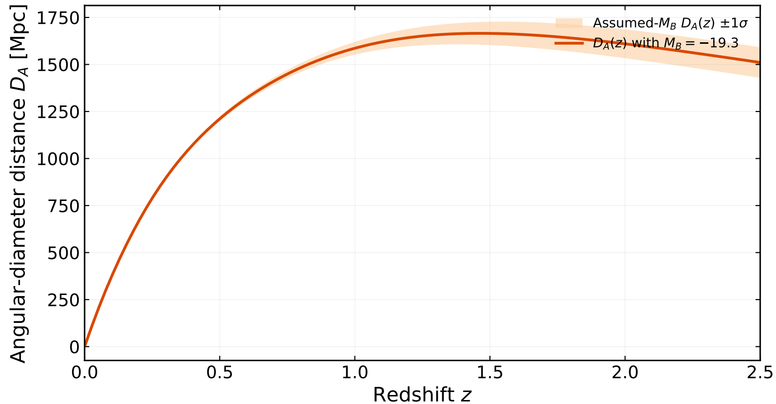
Inferred D_A(z) from reconstructed m_B(z) under fixed M_B
