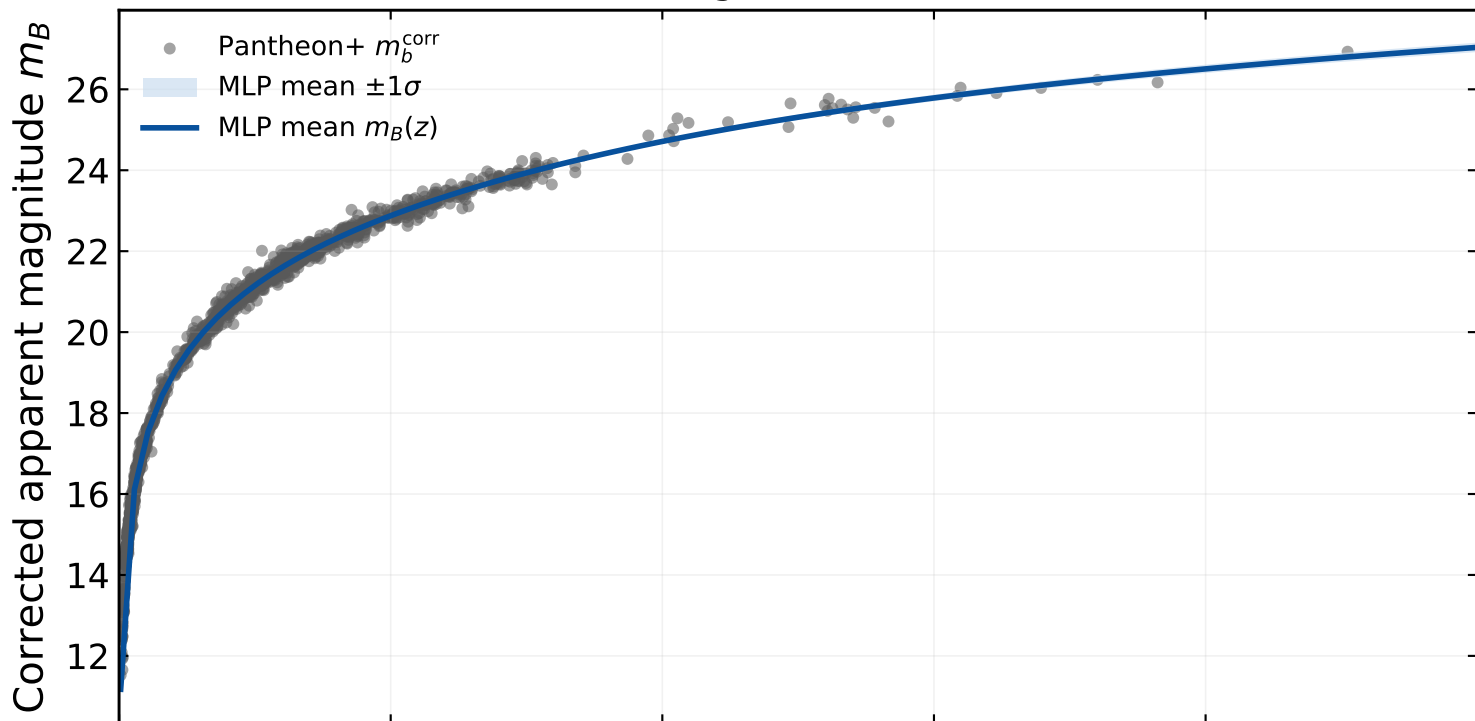
Pantheon+ corrected magnitudes and reconstructed m_B(z)
