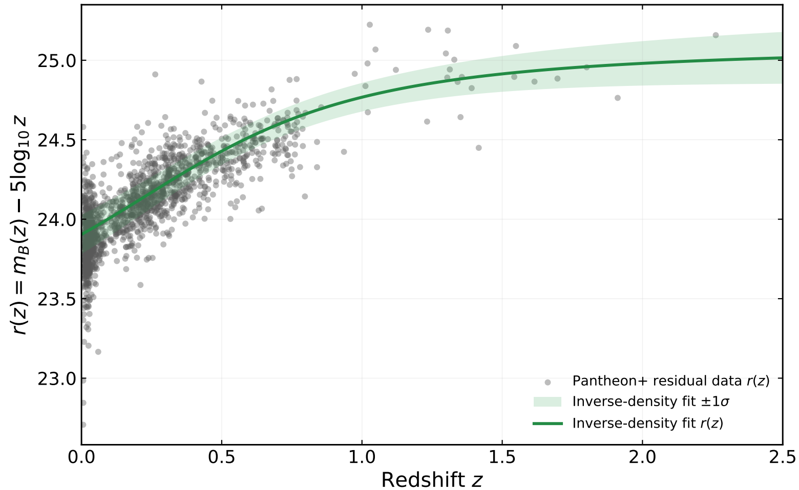
Pantheon+ residuals and inverse-density ANN fit in r(z) space
