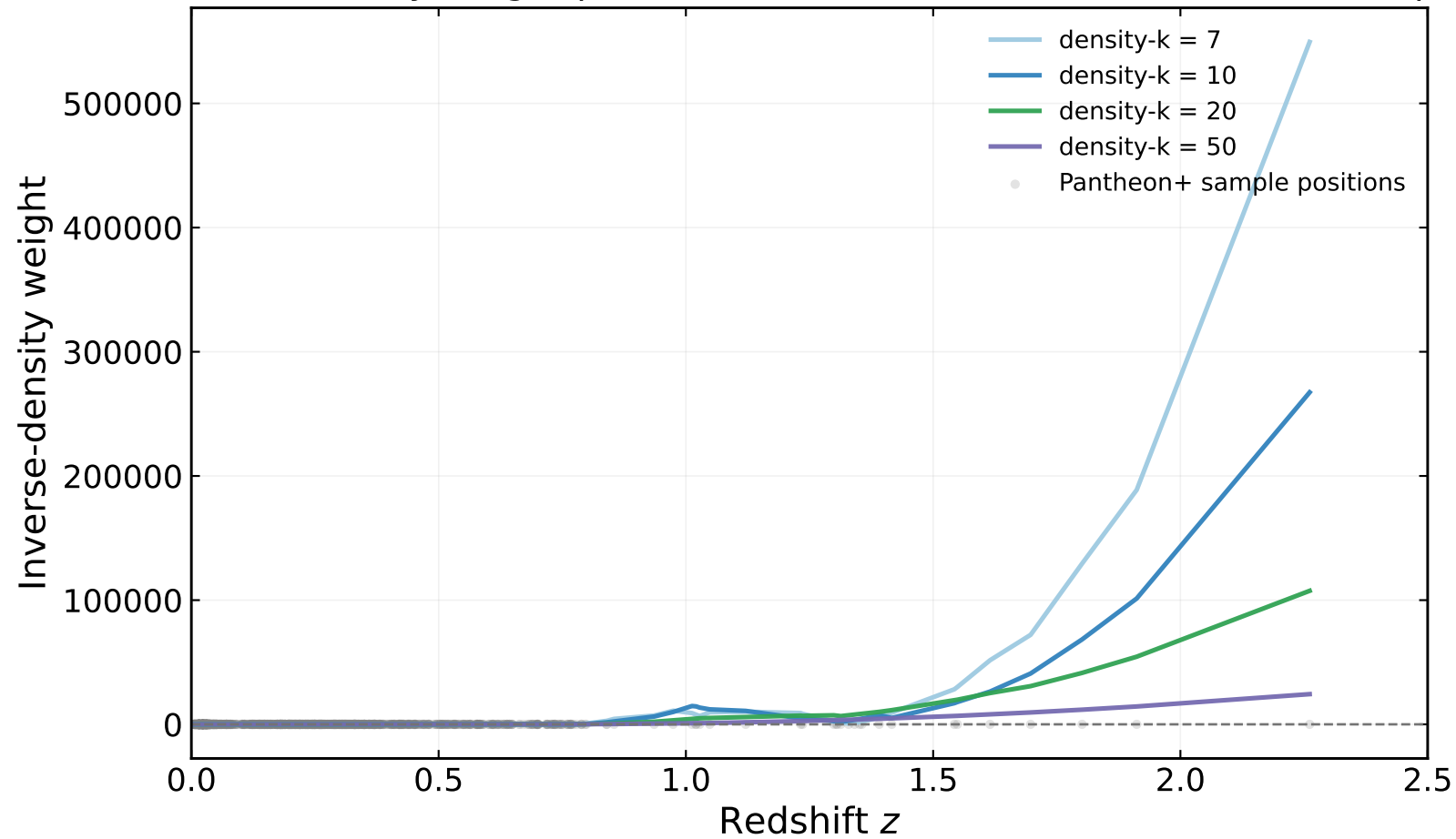
Inverse-density weight profiles on the actual Pantheon+ redshift sample
