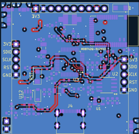
3D render and routed layout
