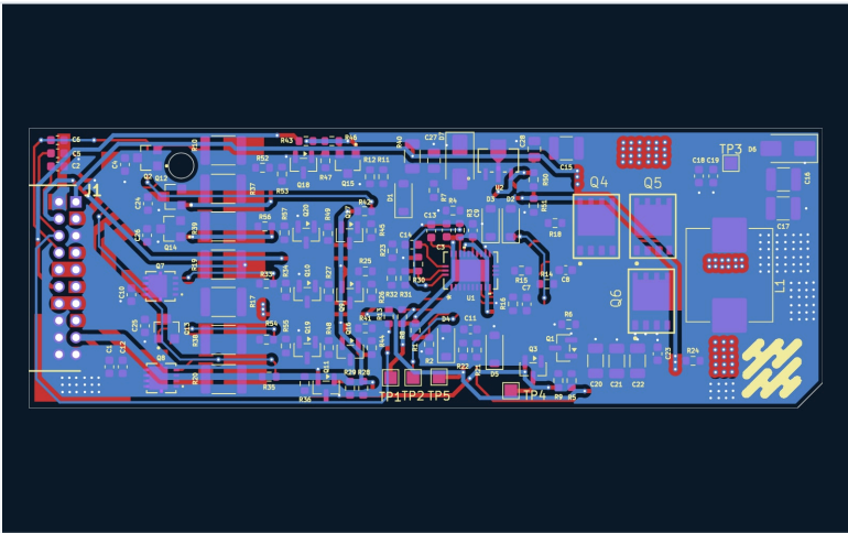
3D render and routed layout
