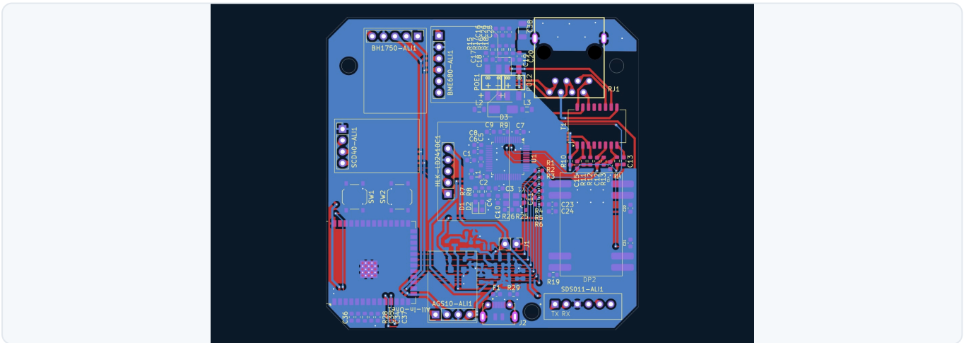
3D render and routed layout
