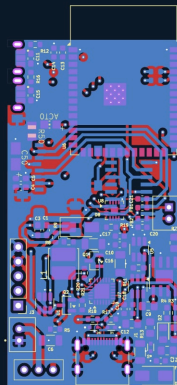
3D render and routed layout
