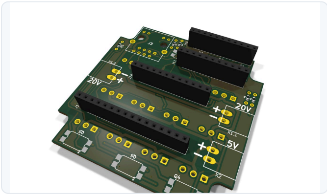
3D render and routed layout
