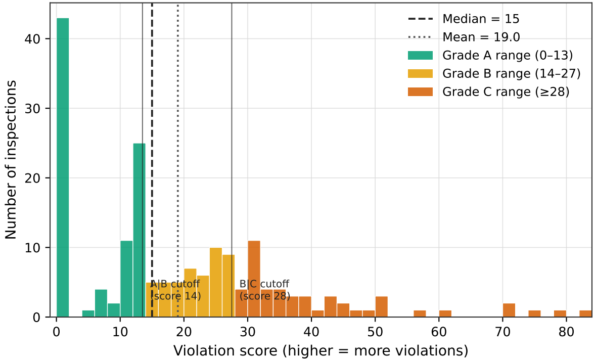
Distribution of NYC restaurant inspection scores, 2016-2025 (n = 180 inspections)
