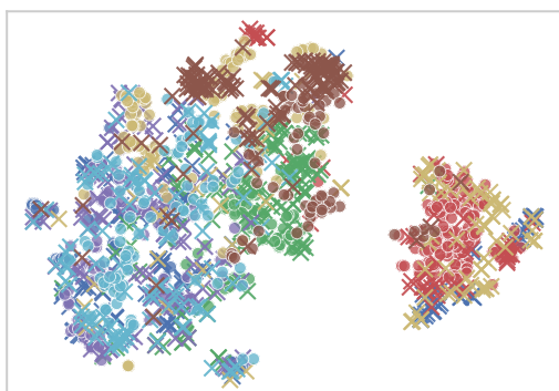
ElectricDevices: Temporal
