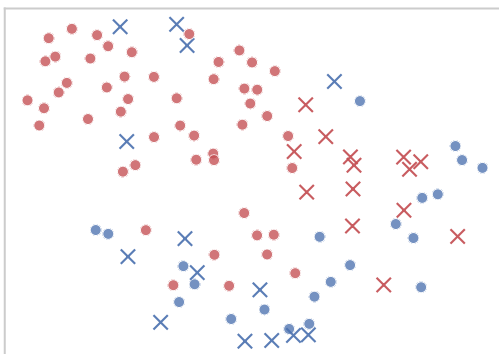
ECG200: Morphology
