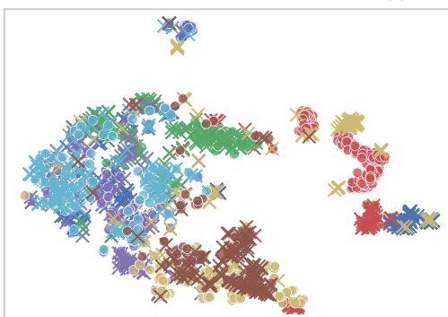
ElectricDevices: Morphology
