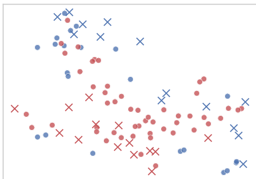
ECG200: Temporal
