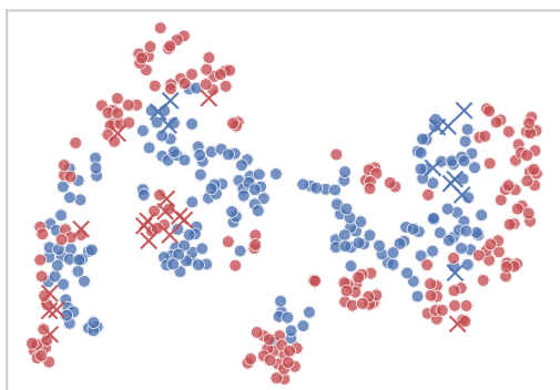
TwoLeadECG: Temporal
