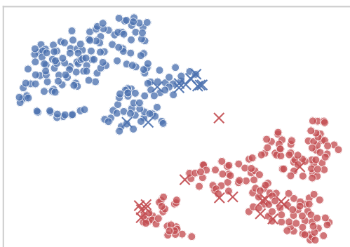
TwoLeadECG: Morphology
