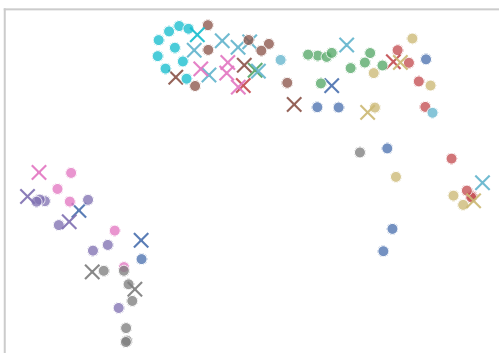
ACSF1: Morphology
