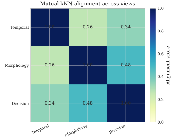
Fig. 6. Mutual k -nearest-neighbor alignment among temporal, morphology, and fused decision representations. Lower temporal–morphology alignment indicates complementary neighborhood structures, while the fused decision state remains aligned with both branches.
