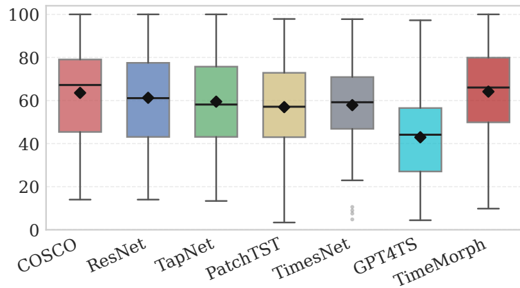
5-shot
