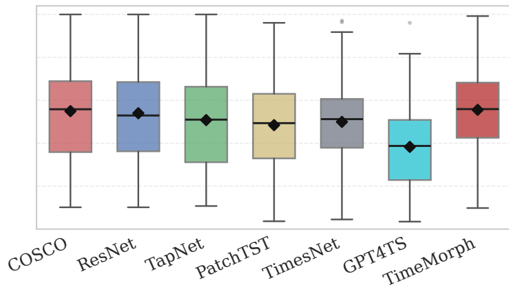
10-shot
