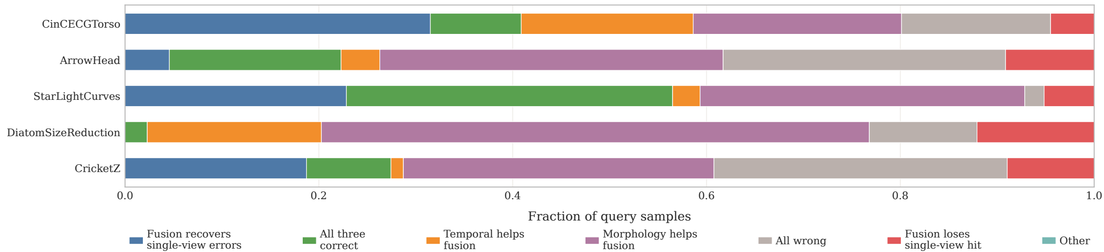
Branch correctness overlap
