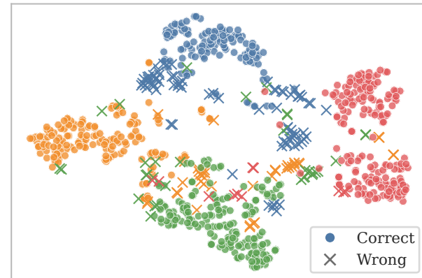
CinCECGTorso: fused LLM decision state
