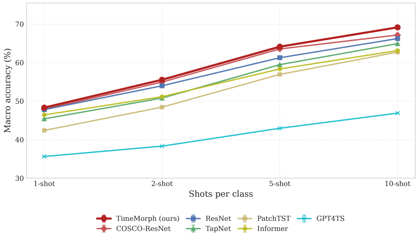
Fig. 8. Shot-scaling trend on the 128 UCR datasets. Each point reports the mean accuracy over five runs. TimeMorph remains the strongest method across all four shot settings.
