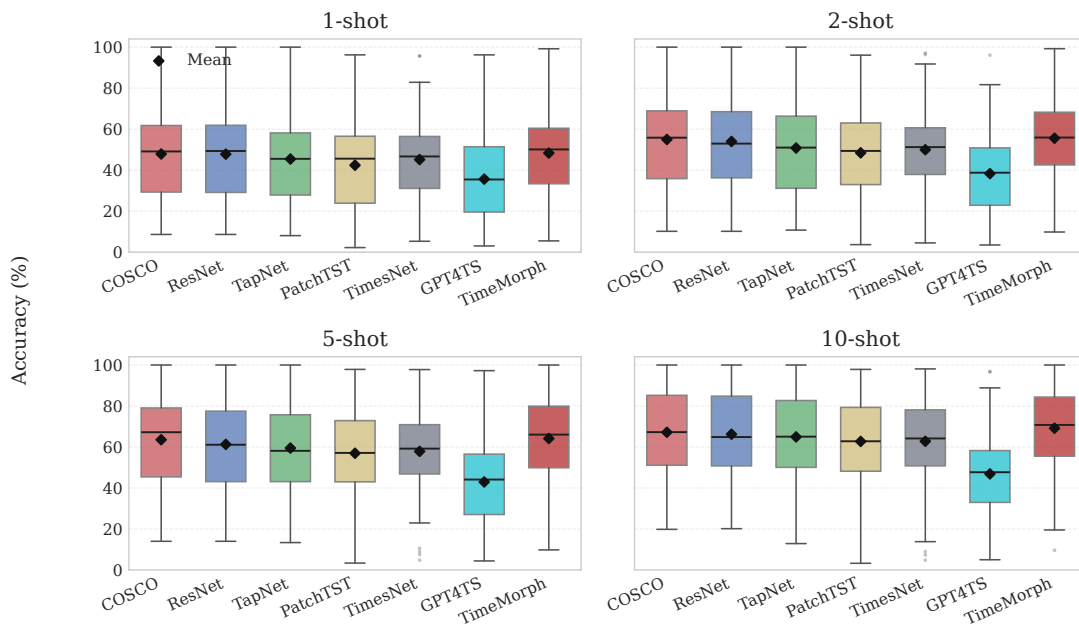
Fig. 7. Per-dataset accuracy distribution on the 128 UCR datasets. Each box summarizes one method's accuracy across datasets for a fixed shot setting; diamonds mark mean accuracies.
