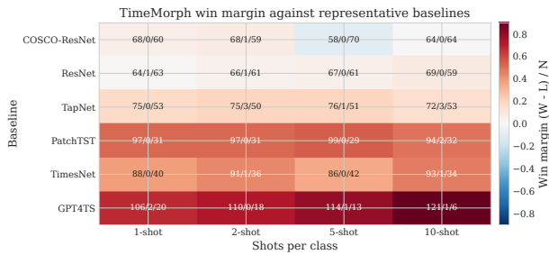
Fig. 6. Win-tie-loss heatmap against representative UCR baselines. Each cell reports wins/ties/losses over 128 datasets, with color indicating the normalized win margin (W - L) / N .
