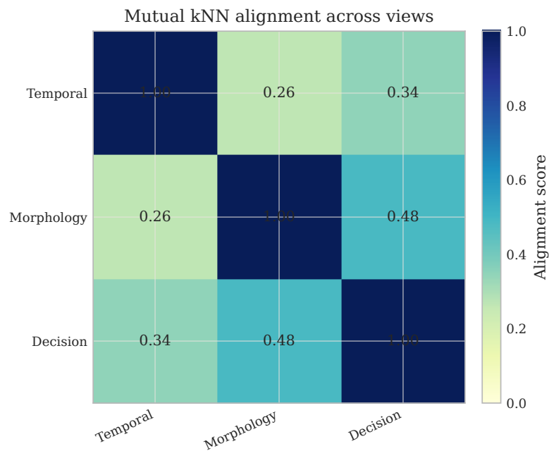
Fig. 10. Mutual k -nearest-neighbor alignment among temporal, morphology, and fused decision representations. The heatmap summarizes neighborhood overlap across the representative qualitative-analysis datasets; lower temporal–morphology alignment indicates different neighborhood structures rather than lower accuracy.
