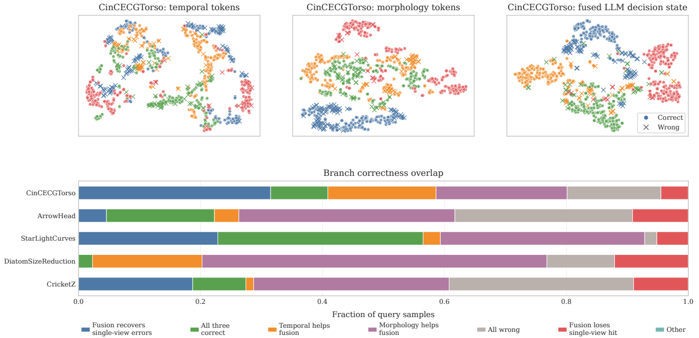
Fig. 5. Representation analysis. The top row gives t-SNE visualizations [57] of temporal, morphology, and fused LLM decision representations. Points are colored by ground-truth class, and misclassified samples are marked separately. The stacked bars compare correctness overlap among temporal-only, morphology-only, and fused dual-view inference on the same fine-tuned checkpoint.
