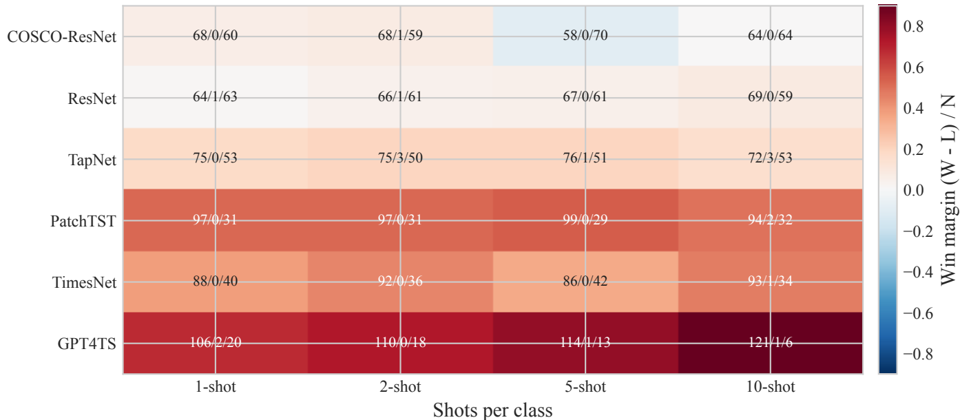
TimeMorph win margin against representative baselines
