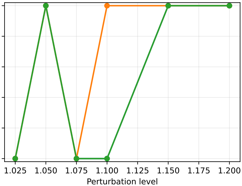
Scale change
