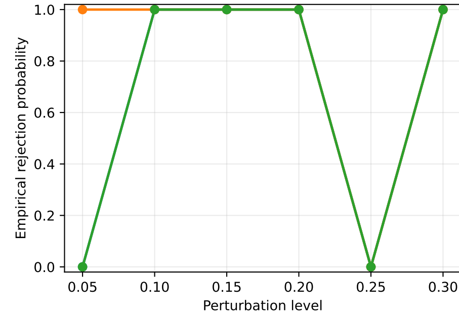
Location shift
