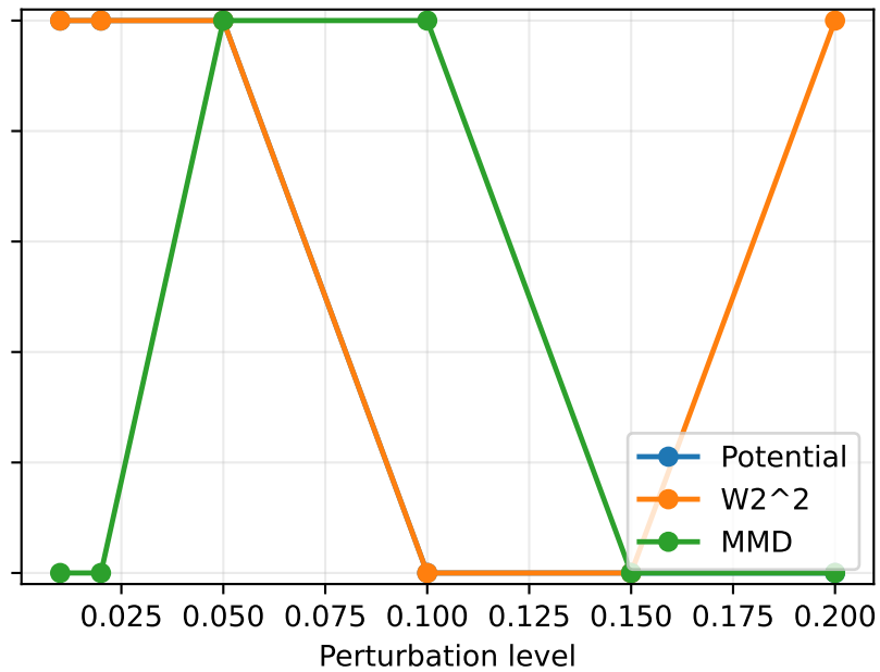
Mixture contamination
