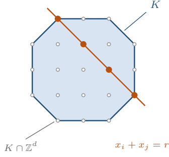
Fig. 2 The exchange fiber of Definition 3.1. On the left, K is a symmetric planar section of the body and the grey dots are the lattice points K \cap \mathbb{Z}^d in it. Fixing the residual coordinates and the sum x_i + x_j = r cuts out the segment drawn in orange; its lattice points, recorded through \delta = x_i - x_j , form a centered interval of one parity class. Here the four marked points have \delta \in \{-3, -1, 1, 3\} , so m = 3 .
