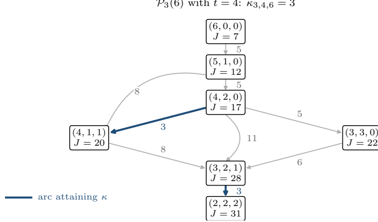
Fig. 8 The unit-transfer graph \mathcal{P}_3(6) for t = 4 . Vertices are the partitions of six into at most three parts, labelled by their lens values J = J_{4,4}^{(3)} ; each arrow is one legal balancing transfer, labelled by its exact increment. All nine weights are positive, which gives stability along any path, and the smallest of them is \kappa_{3,4,6} = 3 , attained exactly on the two highlighted arcs.
