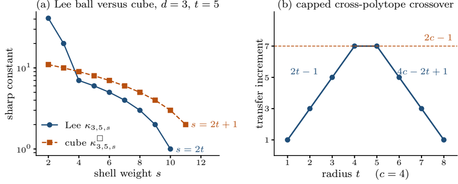
Fig. 11 Quantitative profiles of the two comparisons of this section. Panel (a) plots the Lee constant \kappa_{3,5,s} of Theorem 4.17 against the cube constant \kappa_{3,5,s}^\square of (44) on a logarithmic scale: the cube decays linearly and stays active one shell longer, while the Lee constant drops steeply off the two innermost shells. The labelled markers are the last active shells; beyond them both constants vanish. In d = 3 the two branches of (29) agree on the common value 2t - s + 1 for s \geq 4 , so the even-odd split is visible only from d \geq 4 on. Panel (b) plots the tent of (47) for c = 4 , with the two linear branches meeting at the plateau 2c - 1 carried by t = c and t = c + 1 .
