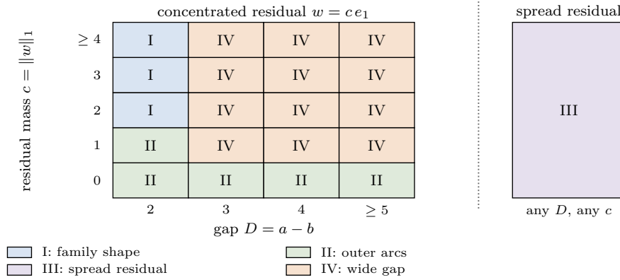
Fig. 9 The partition of Lemma 4.20 in the invariants D = a - b and c = \|w\|_1 . Concentrated residuals w = ce_1 occupy the left panel, where the pair (D, c) alone decides the case; residuals with two or more nonzero coordinates form Case III regardless of (D, c) , shown on the right. Only Case I supports the sharp family.
