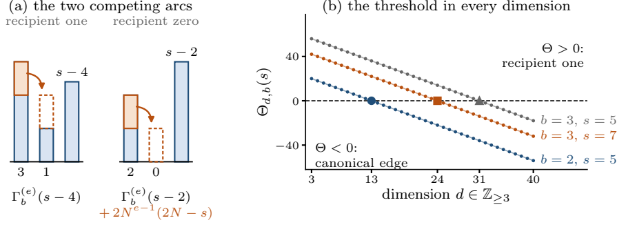
Fig. 12 The competition of Theorem 6.4. In (a) the two candidate arcs of (70) as donor, recipient, and residual coordinates, with bar heights schematic: the shaded unit is the one transferred and the dashed outline is where it lands. The recipient-zero arc buys a larger residual and pays the facet surcharge. In (b) the threshold (72) at every integer dimension for three pairs (b, s) : it decreases with slope -2 , so each pair has a single zero, at which both arcs are minimizing.
