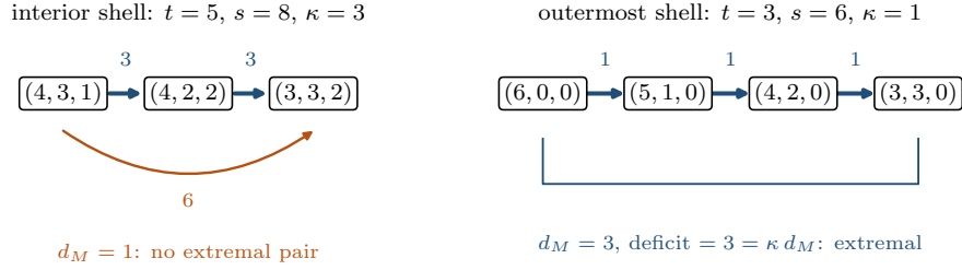
Fig. 10 The concatenation obstruction of Theorem 4.26, in d = 3 . Left, an interior shell: the two consecutive arcs are minimizing, yet their endpoints already lie at transfer distance one, so the chain is not a geodesic and the pair is not extremal. Right, an outermost shell: the two-coordinate path is a geodesic whose every segment is minimizing, and equality in (38) persists at all distances. Arrow labels are lens deficits.
