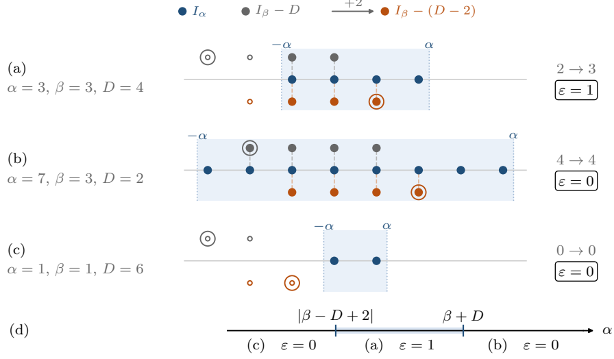
Fig. 3 The three regimes of Lemma 3.3. In (a)–(c) the middle row is I_\alpha , the row above it is I_\beta - D , and the row below is that set translated by two; the shaded strip is the window |x| \leq \alpha , open markers lie outside it, and dashed links mark the coincidences, counted on the right. The translation deletes the endpoint -\beta - D and appends \beta - D + 2 , the two ringed markers, so the count changes by at most one: it rises when the appended endpoint lies in the window while the deleted one did not (a), and is unchanged when both lie inside (b) or both outside (c). The remaining combination cannot occur because |\beta - D + 2| \leq \beta + D . Panel (d) is the partition of the \alpha -axis at fixed \beta and D that the three regimes produce, which is the criterion (5).
