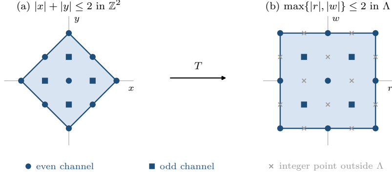
Fig. 5 The diamond-to-square map. T(x, y) = (x + y, x - y) is a bijection of \mathbb{Z}^2 onto \Lambda = \{(r, w) \in \mathbb{Z}^2 : r \equiv w \pmod{2}\} , not onto \mathbb{Z}^2 : the crosses in (b) are the integer points it misses. Discs and squares mark the channels r even and r odd, which the map keeps separate.
