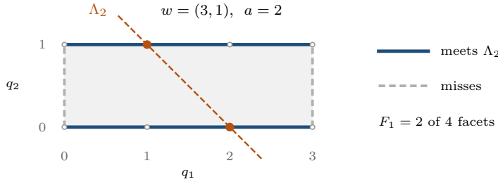
Fig. 7 The incidence bound of Lemma 4.12 for h = 2 and w = (3, 1) , so c = 4 and a = 2 . A facet misses \Lambda_2 exactly when the coordinate it freezes is too heavy, here q_1 = 0 and q_1 = 3 ; the other two meet it, matching 2^1 \binom{h-1}{1} = 2 . Neither vertex meets the layer, matching 2^2 \binom{h-1}{2} = 0 .
