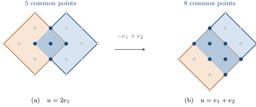
Fig. 4 A unit balancing transfer and what it does to the lens. Both shifts lie on the shell \|u\|_1 = 2 and differ by one unit moved from the larger coordinate to the smaller one. In each panel the blue diamond is B_1^2(2) , the orange one is B_1^2(2) - u , and the filled points are the lattice points they share; the count rises from five to eight.
