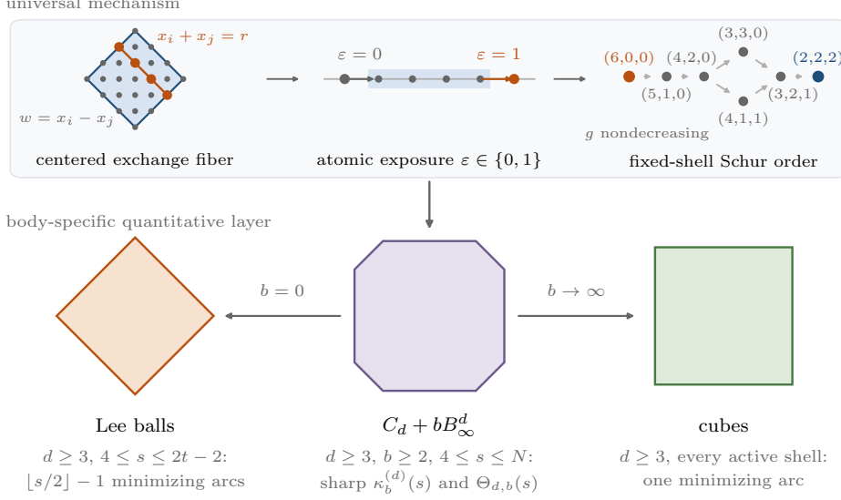
Fig. 1 Logical architecture; the bodies are two-dimensional schematics. Above: a centered exchange fiber, the straight slice on which the other coordinates and r = x_i + x_j are fixed while w = x_i - x_j varies; the atomic exposure \varepsilon \in \{0, 1\} of one balancing transfer, according to whether the moved endpoint leaves the opposite interval; and the order their sum produces on a fixed shell, drawn as the majorization Hasse diagram of s = 6 in d = 3 and oriented from skewed to balanced, the direction along which g does not decrease. Below: the quantitative layer, which is body-dependent. The structural theorem of Section 6 evaluates it on the interpolating family C_d + bB_\infty^d and recovers equal Lee balls and equal cubes as the two degenerate regimes, the cases without factorization and without surcharge; the Lee count is that of the interior shells 4 \leq s \leq 2t - 2 .
