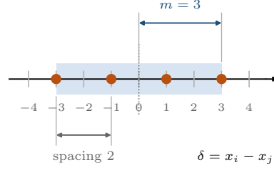
Fig. 2 The exchange fiber of Definition 3.1. On the left, K is a symmetric planar section of the body and the grey dots are the lattice points K \cap \mathbb{Z}^d in it. Fixing the residual coordinates and the sum x_i + x_j = r cuts out the segment drawn in orange; its lattice points, recorded through \delta = x_i - x_j , form a centered interval of one parity class. Here the four marked points have \delta \in \{-3, -1, 1, 3\} , so m = 3 .
