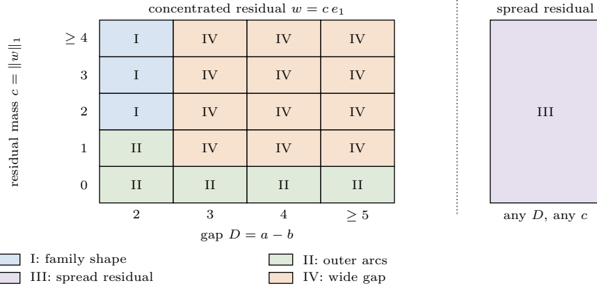
Fig. 9 The partition of Lemma 4.20 in the invariants D = a - b and c = \|w\|_1 . Concentrated residuals w = ce_1 occupy the left panel, where the pair (D, c) alone decides the case; residuals with two or more nonzero coordinates form Case III regardless of (D, c) , shown on the right. Only Case I supports the sharp family.
