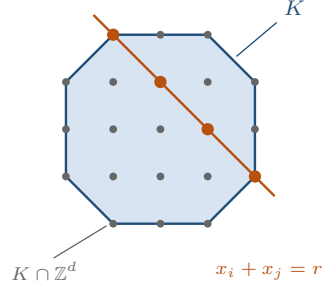
Fig. 2 The exchange fiber of Definition 3.1. On the left, K is a symmetric planar section of the body and the grey dots are the lattice points K \cap \mathbb{Z}^d in it. Fixing the residual coordinates and the sum x_i + x_j = r cuts out the segment drawn in orange; its lattice points, recorded through \delta = x_i - x_j , form a centered interval of one parity class. Here the four marked points have \delta \in \{-3, -1, 1, 3\} , so m = 3 .
