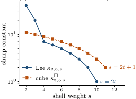
(a) Lee ball versus cube, d = 3 , t = 5
