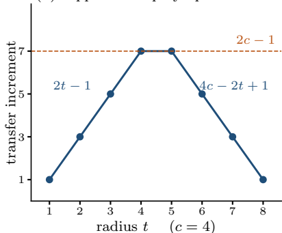
(b) capped cross-polytope crossover
