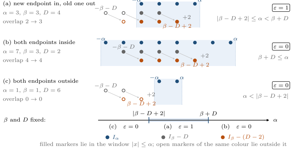
Fig. 3 The three regimes of Lemma 3.3, each drawn with its own (\alpha, \beta, D) . Translating the whole interval I_\beta - D by two deletes its left endpoint -\beta - D and appends the right endpoint \beta - D + 2 , so the overlap with I_\alpha can grow by at most one point. It grows when the new endpoint lies in the window |x| \leq \alpha while the deleted one did not (a), and is unchanged when both lie inside (b) or both outside (c); the fourth combination cannot occur because |\beta - D + 2| \leq \beta + D . The bottom line is the partition of the \alpha -axis at fixed \beta and D that these three regimes produce, which is the criterion (5).
