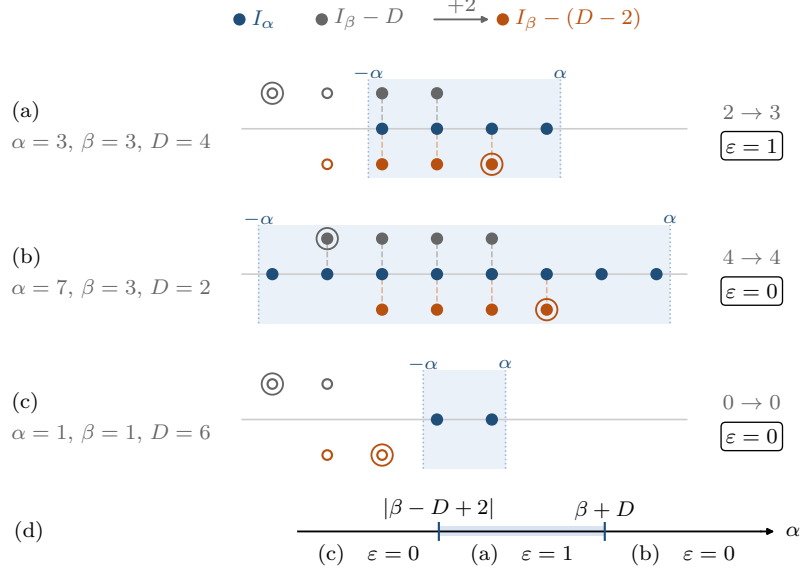
Fig. 3 The three regimes of Lemma 3.3. In (a)–(c) the middle row is I_\alpha , the row above it is I_\beta - D , and the row below is that set translated by two; the shaded strip is the window |x| \leq \alpha , open markers lie outside it, and dashed links mark the coincidences, counted on the right. The translation deletes the endpoint -\beta - D and appends \beta - D + 2 , the two ringed markers, so the count changes by at most one: it rises when the appended endpoint lies in the window while the deleted one did not (a), and is unchanged when both lie inside (b) or both outside (c). The remaining combination cannot occur because |\beta - D + 2| \leq \beta + D . Panel (d) is the partition of the \alpha -axis at fixed \beta and D that the three regimes produce, which is the criterion (5).
