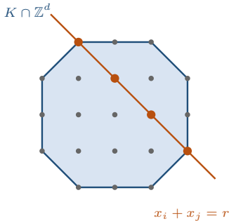
(a) a fixed coordinate-sum line
