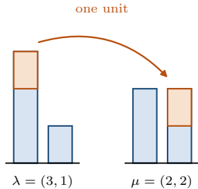
(b) the same move as a transfer
