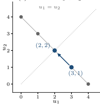
(a) one shell u_1 + u_2 = 4
