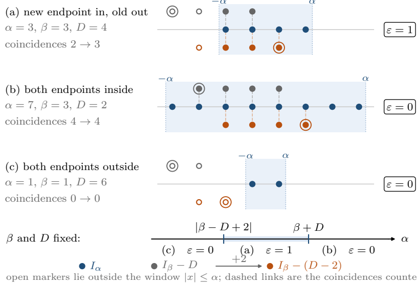
Fig. 3 The three regimes of Lemma 3.3, each with its own (\alpha, \beta, D) . In every panel the middle row is I_\alpha , the row above it is I_\beta - D , and the row below is that set translated by two; dashed links mark the points each overlap counts. The translation deletes the endpoint -\beta - D and appends \beta - D + 2 , the two ringed markers, so the count changes by at most one. It rises when the appended endpoint lies in the window |x| \leq \alpha while the deleted one did not (a), and is unchanged when both lie inside (b) or both outside (c); the fourth combination cannot occur because |\beta - D + 2| \leq \beta + D . The bottom line is the partition of the \alpha -axis at fixed \beta and D that these three regimes produce, which is the criterion (5).
