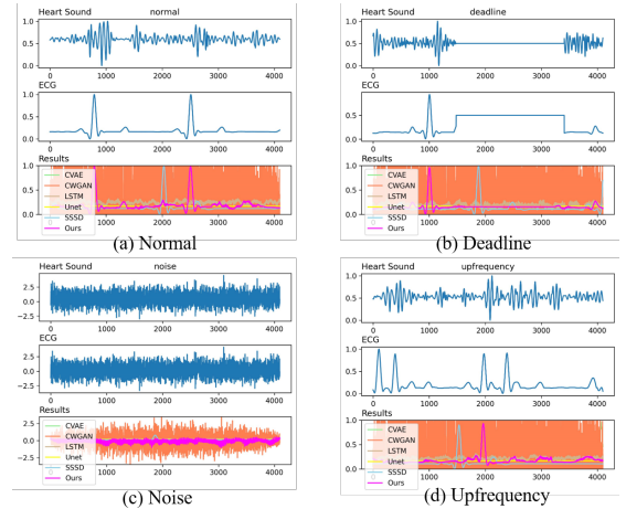
Fig. 3. Visualisation of ECGs generated by different methods under different kinds of datasets.
