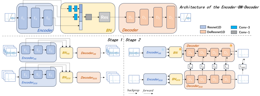
Fig. 2. Framework Overview: The upper section shows the encoder-bottleneck-decoder architecture, where the bottleneck aligns multi-scale features from different encoder layers to compact features, remove redundancy, and improve decoding. The lower section outlines two training phases: pre-training, where the model generates its own signals, and distillation, where the Radar2ECG decoder learns ECG generation from the ECG decoder, with adjustments to the bottleneck to support feature transformation.
