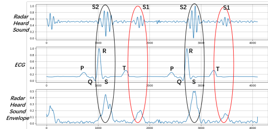
Fig. 1. Visualization of the "coarse-grained" relationship between radar heart sound and synchronized ECG signals shows that the S1 wave of the heart sound correlates with the onset of the P wave after the ECG's T wave, while the S2 wave correlates with the onset of the S wave after the R wave.
