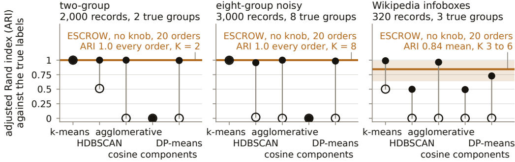
Figure 4: Tuned baselines against ESCROW on three streams, scored by ARI. Filled markers are oracle scores (knob chosen on the test labels), open markers transferred scores (knob tuned on another stream, worse of two transfers), the grey line the drop: to 0.0 for agglomerative and DP-means on the synthetic streams and to at most 0.0017 for every transferred knob on Wikipedia; k -means has no knob, filled handed the true K , open picking K by silhouette. ESCROW (gold), nothing calibrated and no embedding: ARI 1.0 on all 20 orders of both synthetic streams; on Wikipedia mean 0.84 over 20 orders, range 0.64 to 0.99, K 3 to 6 (results/e4_first_tier.json, results/e5_order_dependence.json).
