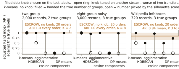
Figure 8: Tuned baselines against ESCROW on three streams, scored by ARI. Filled markers are or-acle scores, with the knob chosen on the test labels, and open markers are transferred scores, with the knob tuned on another stream, the worse of two transfers. The grey line is the drop between them: to 0.0 for agglomerative and DP-means on the synthetic streams, and to at most 0.0017 for every transferred knob on Wikipedia. k -means has no knob, so filled is handed the true K and open picks K by silhouette. ESCROW (gold) has nothing calibrated and no embedding (results/e4_first_tier.json, results/e5_order_dependence.json).
