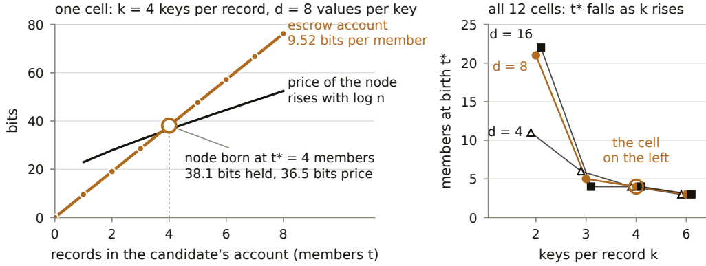
Figure 6: How a node is born. Left: one cell of the two-group fixture, four keys per record and eight values per key, one seed; the account (gold) rises at 9.52 bits per member, the price (ink) with the log of the stream, and the node is born at four members, never before. Right: members at birth across all twelve (k, d) cells fall as k rises, from 11 to 22 at k = 2 to 3 at k = 6 (results/e9_support_curve.json).
