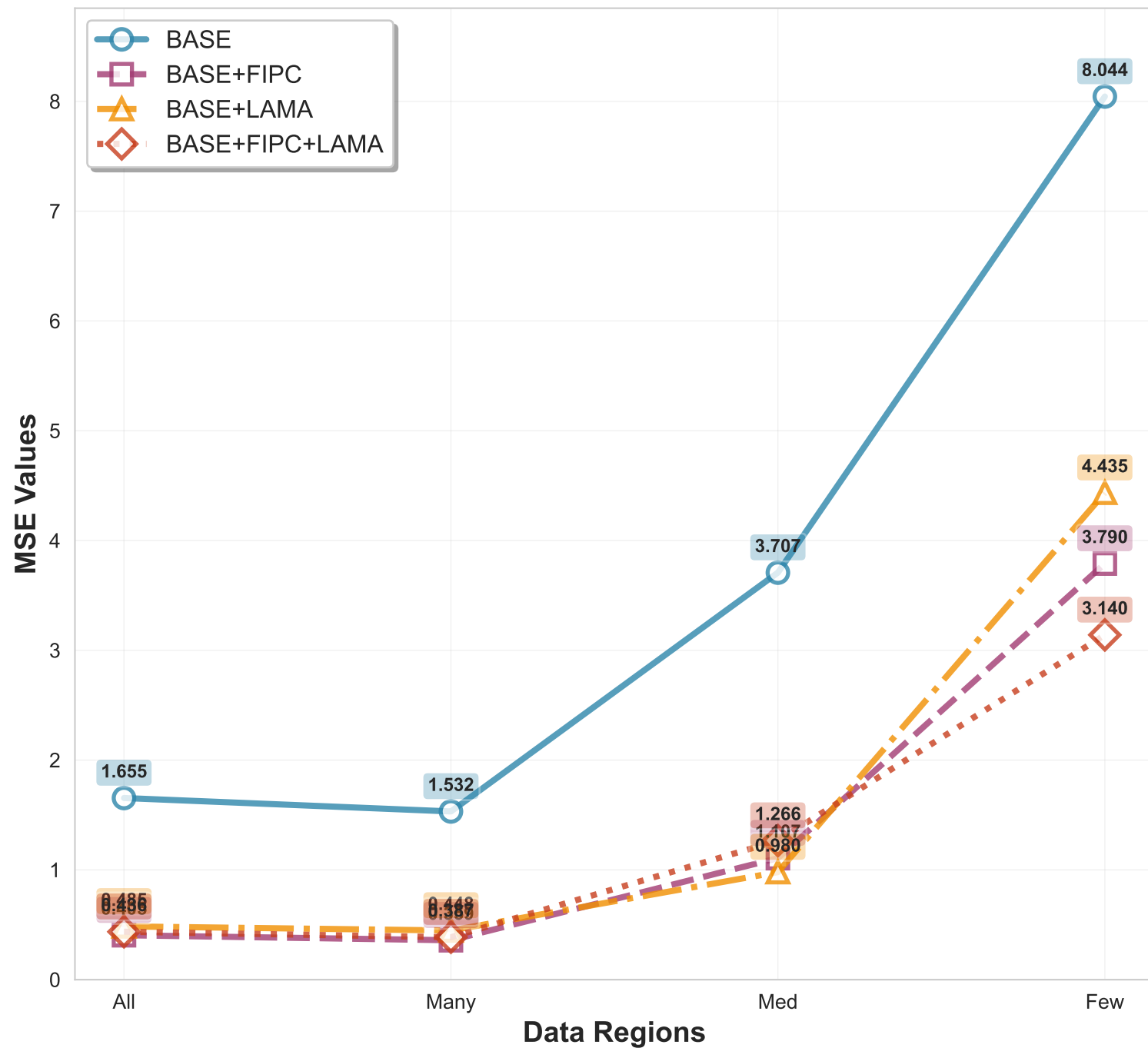
Wine Quality Prediction Ablation Study Results
