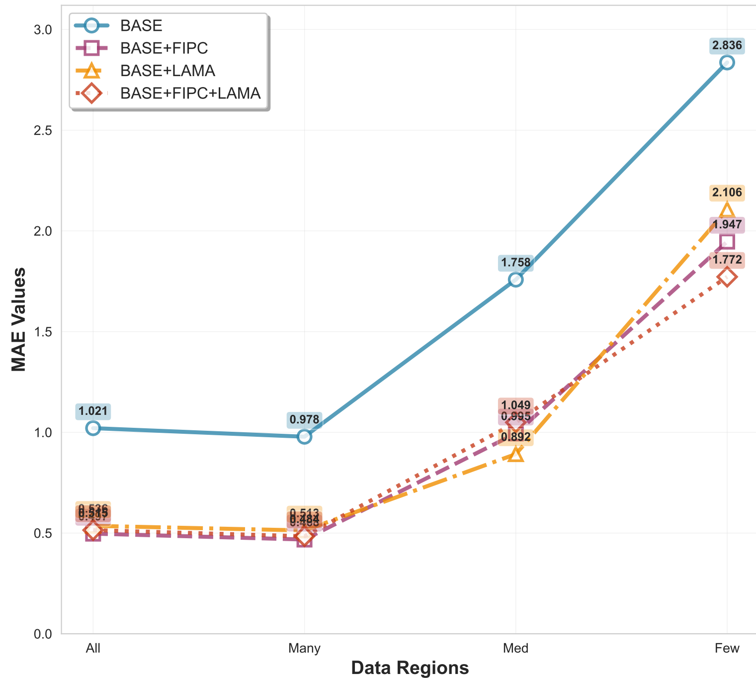
Wine Quality Prediction Ablation Study Results
