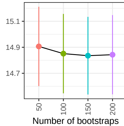
PAAD
