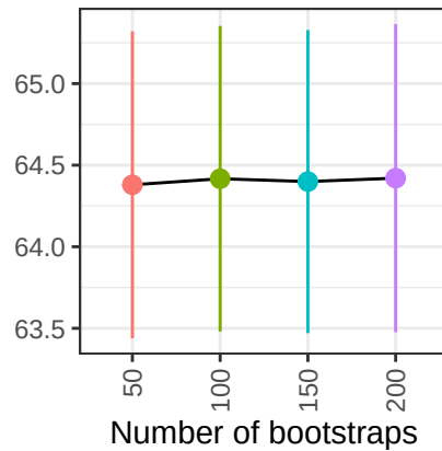
LUSC
