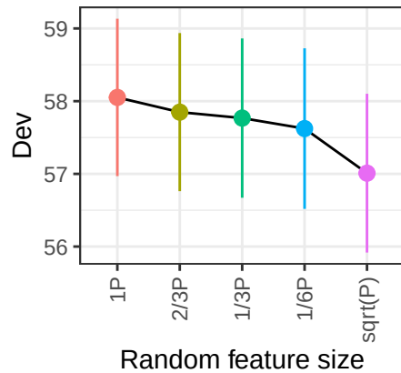
LUSC
