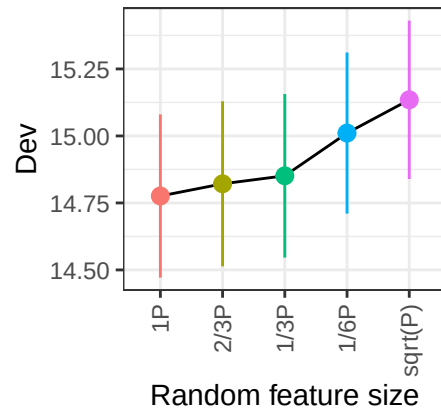
PAAD
