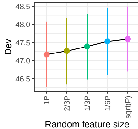
SKCM
