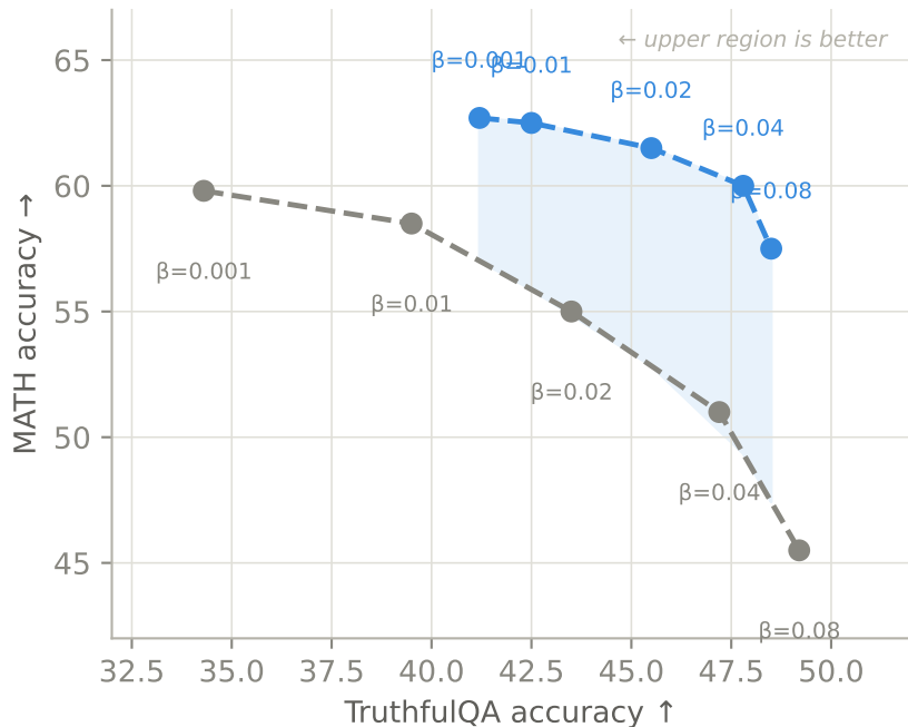
MATH accuracy vs. factual reliability
