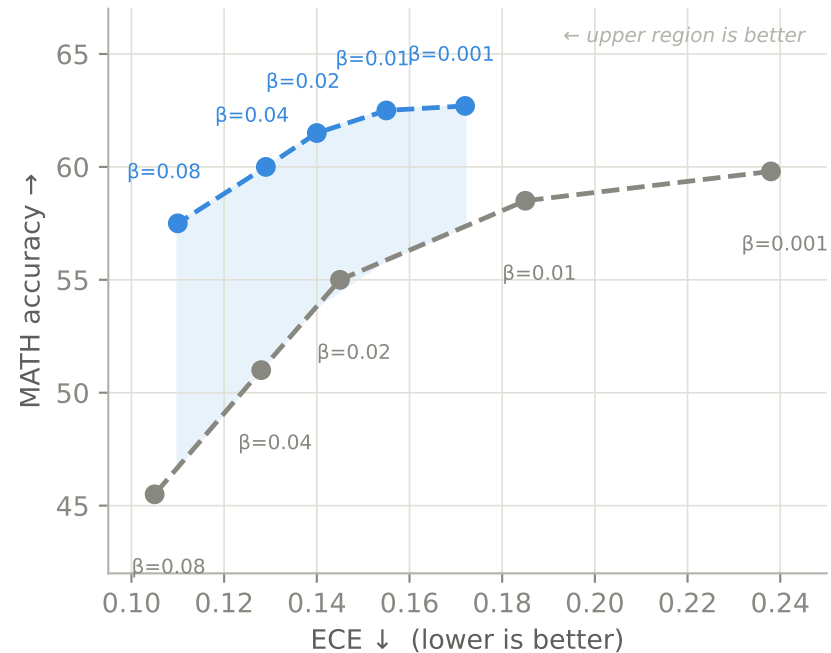
MATH accuracy vs. calibration error
